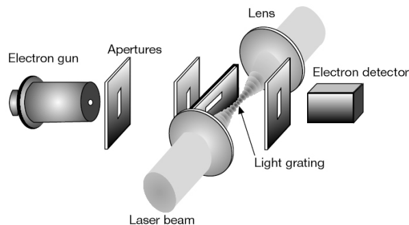
Figure 1. Schematic of our apparatus. Electrons are collimated by four molybdenum slits and diffract from a standing wave of light formed by two counter-propagating laser beams. The electrons must be described by a quantum mechanical wave while the standing light wave acts as a grating.
