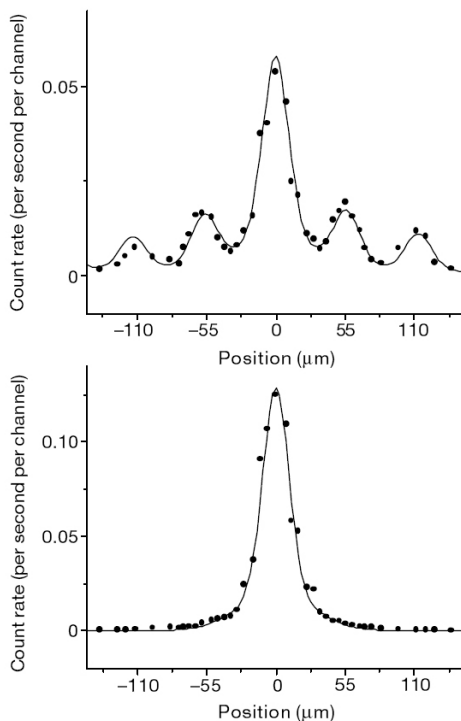
Figure 2. Experimental data. The electron detection rate is presented as a function of detector position. Our data (black points) agree reasonably well with anumerical solution of the Schrdinger equation (described in the text) and clearly show diffraction peaks, which is the signature of the Kapitza-Dirac effect. The bottom figure shows the electron beam profile with the laser beams turned off.
