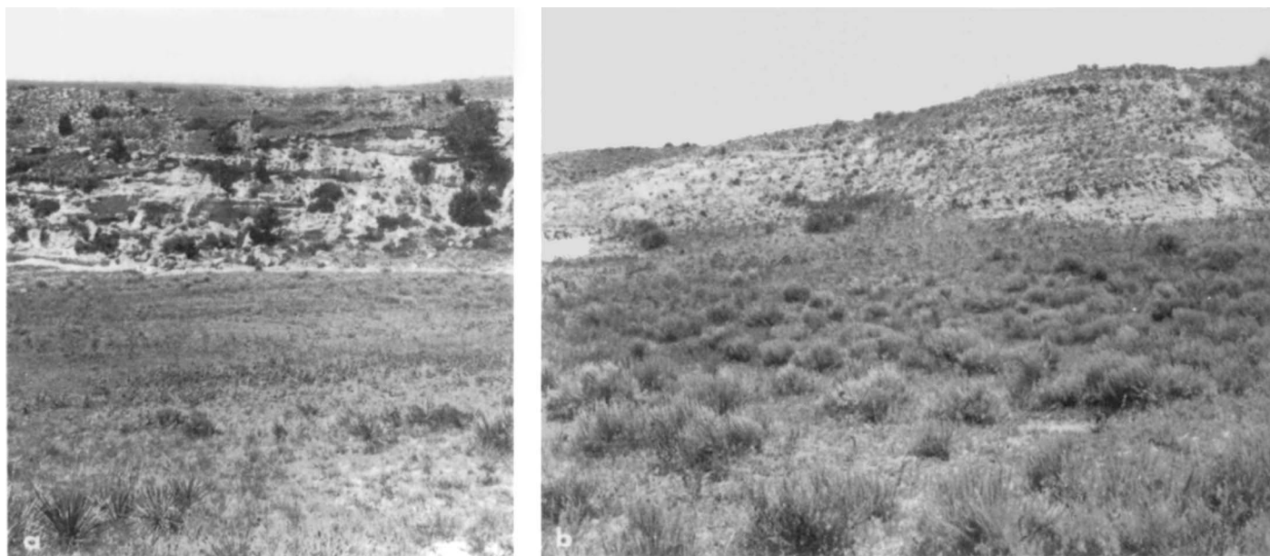
FIGURE 2. a. View from south of Coumbe Bluff looking west at strata of the Ogallala Group dipping toward the northwest. b. View from the same point looking east at a part of the Whitney Member of the Brule Formation containing concretions and at the overlying basal portion of the Ogallala Group. The strata and contact are dipping toward the northwest.
