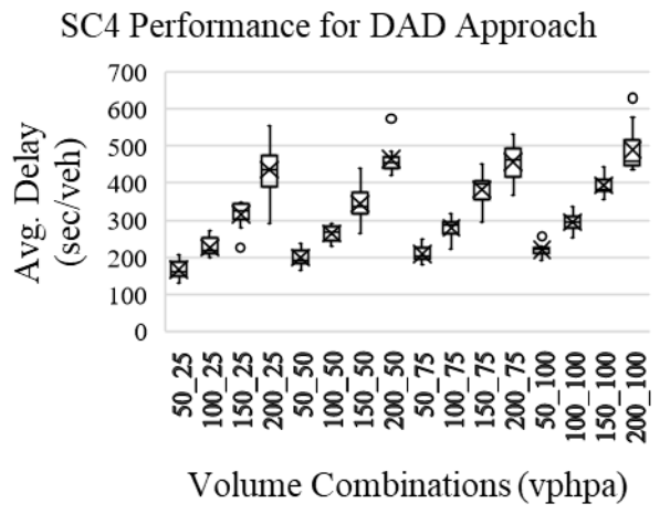
Figure A.4 Average delay for All, Main and DAD approach under SC3 and SC4 for Main approach volume increase for various levels of constant DAD approach volume (WZL=1.1 mile, N_{DAD}=1 , T_{M\%}=20 , T_{DAD\%}=5 )
