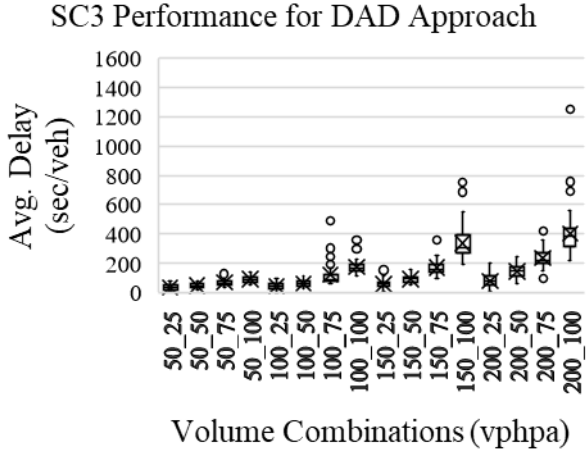
Figure C.2 Average delay for All, Main and DAD approach under SC3 and SC4 for DAD approach volume increase for various levels of constant Main approach volume (WZL=1.1 mile, N_{DAD}=5 , T_{M\%}=20 , T_{DAD\%}=5 )
