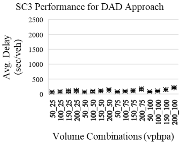
Figure B.4 Average delay for All, Main and DAD approach under SC3 and SC4 for Main approach volume increase for various levels of constant DAD approach volume (WZL=1.1 mile, N_{DAD}=3 , T_{M\%}=20 , T_{DAD\%}=5 )
