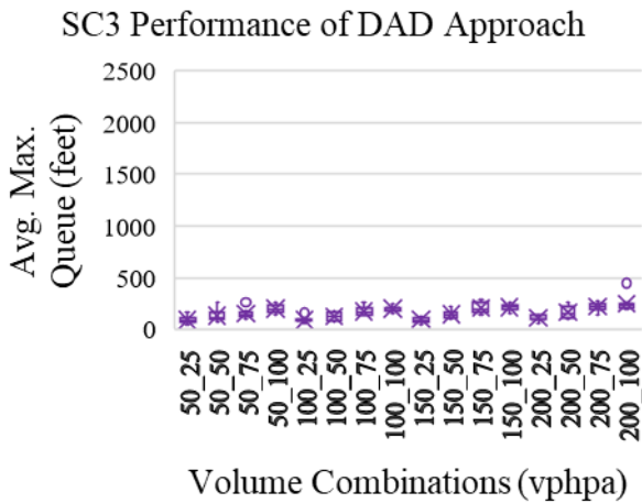
Figure A.6 Average maximum queue for All, Main and DAD approach under SC3 and SC4 for DAD approach volume increase for various levels of constant Main approach volume (WZL=1.1 mile, N_{DAD}=1 , T_{M\%}=20 , T_{DAD\%}=5 )
