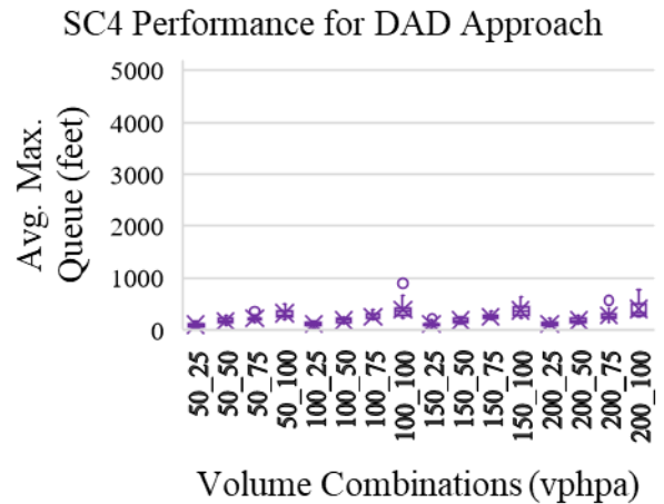
Figure B.6 Average maximum queue for All, Main and DAD approach under SC3 and SC4 for DAD approach volume increase for various levels of constant Main approach volume (WZL=1.1 mile, N_{DAD}=3 , T_{M\%}=20 , T_{DAD\%}=5 )
