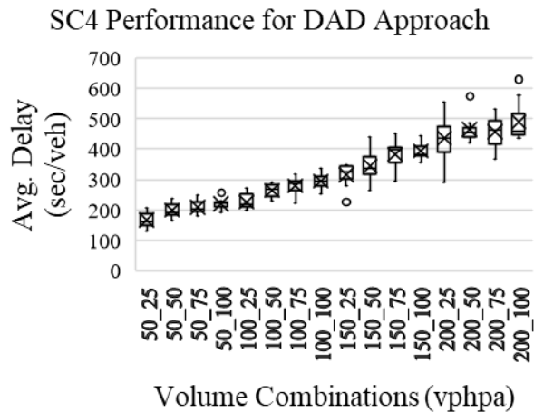
Figure A.2 Average delay for All, Main and DAD approach under SC3 and SC4 for DAD approach volume increase for various levels of constant Main approach volume (WZL=1.1 mile, N_{DAD}=1 , T_{M\%}=20 , T_{DAD\%}=5 )
