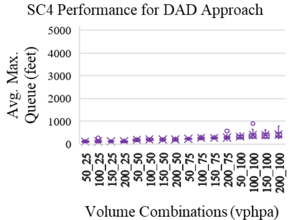
Figure B.8 Average maximum queue for All, Main and DAD approach under SC3 and SC4 for Main approach volume increase for various levels of constant DAD approach volume (WZL=1.1 mile, N_{DAD}=3 , T_{M\%}=20 , T_{DAD\%}=5 )
