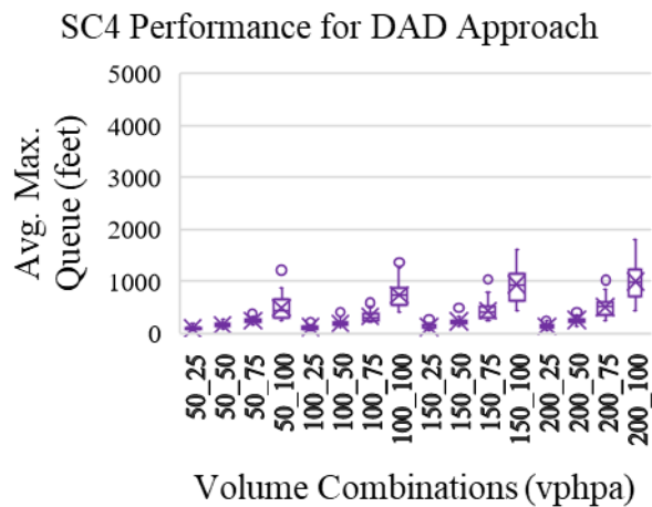
Figure C.8 Average maximum queue for All, Main and DAD approach under SC3 and SC4 for Main approach volume increase for various levels of constant DAD approach volume (WZL=1.1 mile, N_{DAD}=5 , T_M\%=20 , T_{DAD}\%=5 )
