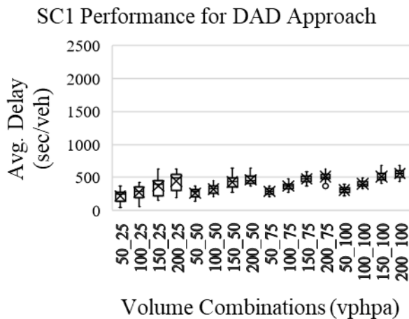
Figure B.3 Average delay for All, Main and DAD approach under SC1 and SC2 for Main approach volume increase for various levels of constant DAD approach volume (WZL=1.1 mile, N_{DAD}=3 , T_{M\%}=20 , T_{DAD\%}=5 )
