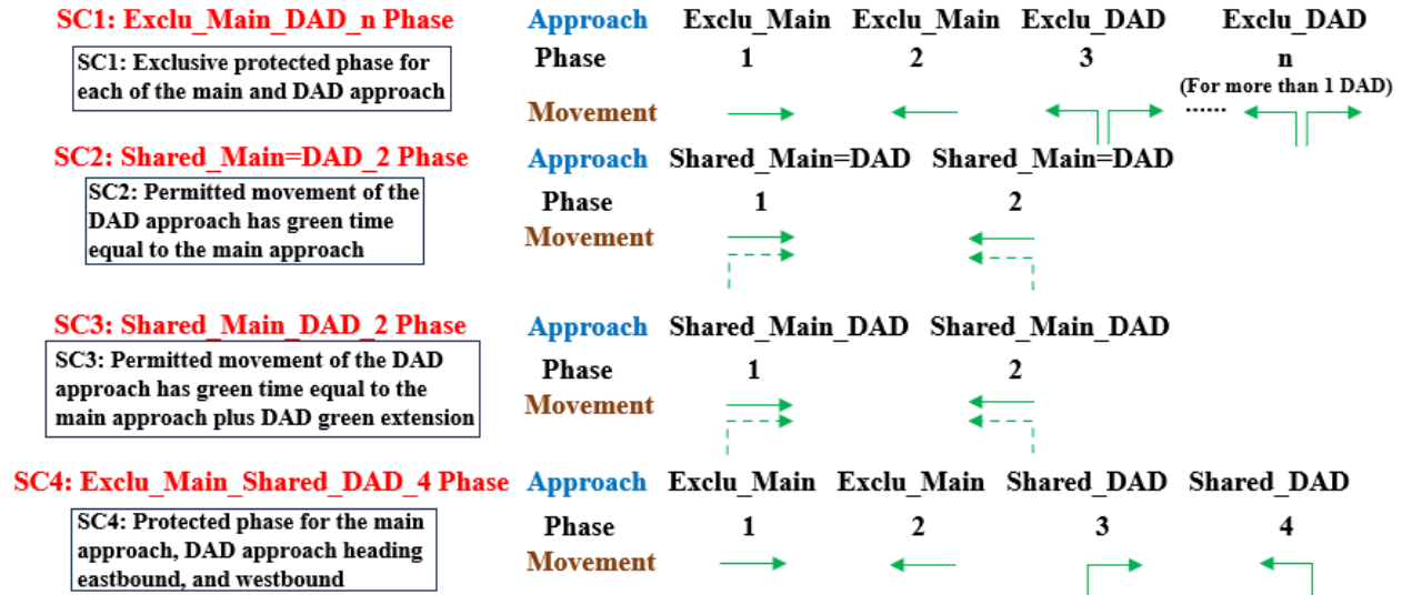
Figure 4.1 Phase and movement of four signal control strategies for DAD-operated work zone
