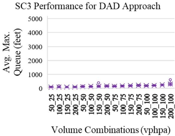
Figure B.8 Average maximum queue for All, Main and DAD approach under SC3 and SC4 for Main approach volume increase for various levels of constant DAD approach volume (WZL=1.1 mile, N_{DAD}=3 , T_{M\%}=20 , T_{DAD\%}=5 )
