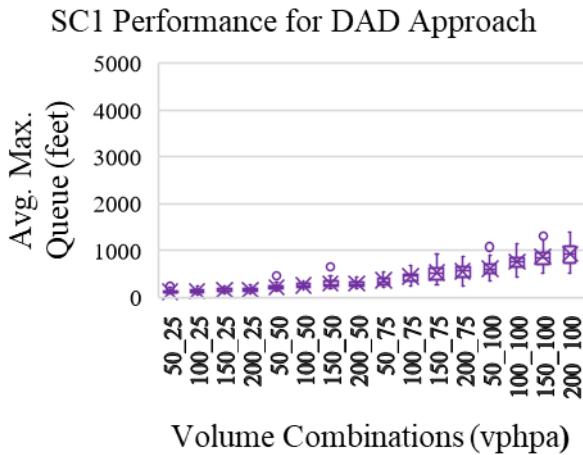
Figure C.7 Average maximum queue for All, Main and DAD approach under SC1 and SC2 for Main approach volume increase for various levels of constant DAD approach volume (WZL=1.1 mile, N_{DAD}=5 , T_{M\%}=20 , T_{DAD\%}=5 )
