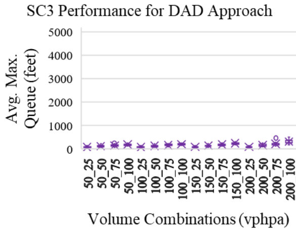
Figure B.6 Average maximum queue for All, Main and DAD approach under SC3 and SC4 for DAD approach volume increase for various levels of constant Main approach volume (WZL=1.1 mile, N_{DAD}=3 , T_{M\%}=20 , T_{DAD\%}=5 )
