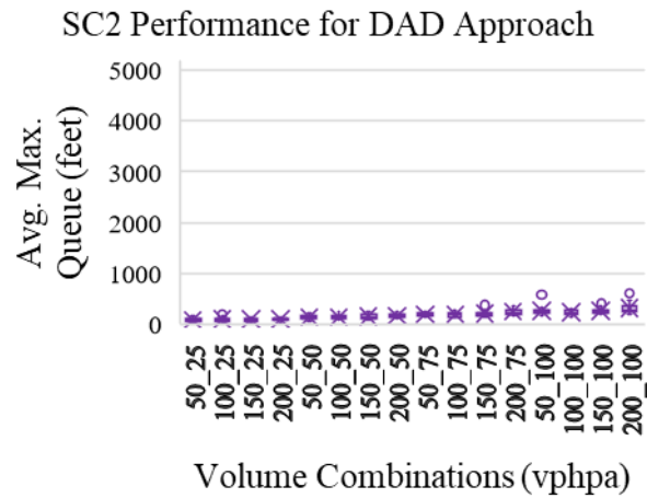
Figure B.7 Average maximum queue for All, Main and DAD approach under SC1 and SC2 for Main approach volume increase for various levels of constant DAD approach volume (WZL=1.1 mile, N_{DAD}=3 , T_{M\%}=20 , T_{DAD\%}=5 )
