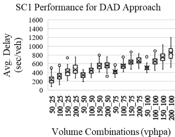
Figure C.3 Average delay for All, Main and DAD approach under SC1 and SC2 for Main approach volume increase for various levels of constant DAD approach volume (WZL=1.1 mile, N_{DAD}=5 , T_{M\%}=20 , T_{DAD\%}=5 )
