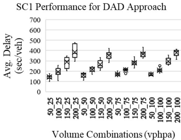
Figure A.3 Average delay for All, Main and DAD approach under SC1 and SC2 for Main approach volume increase for various levels of constant DAD approach volume (WZL=1.1 mile, N_{DAD}=1 , T_{M\%}=20 , T_{DAD\%}=5 )
