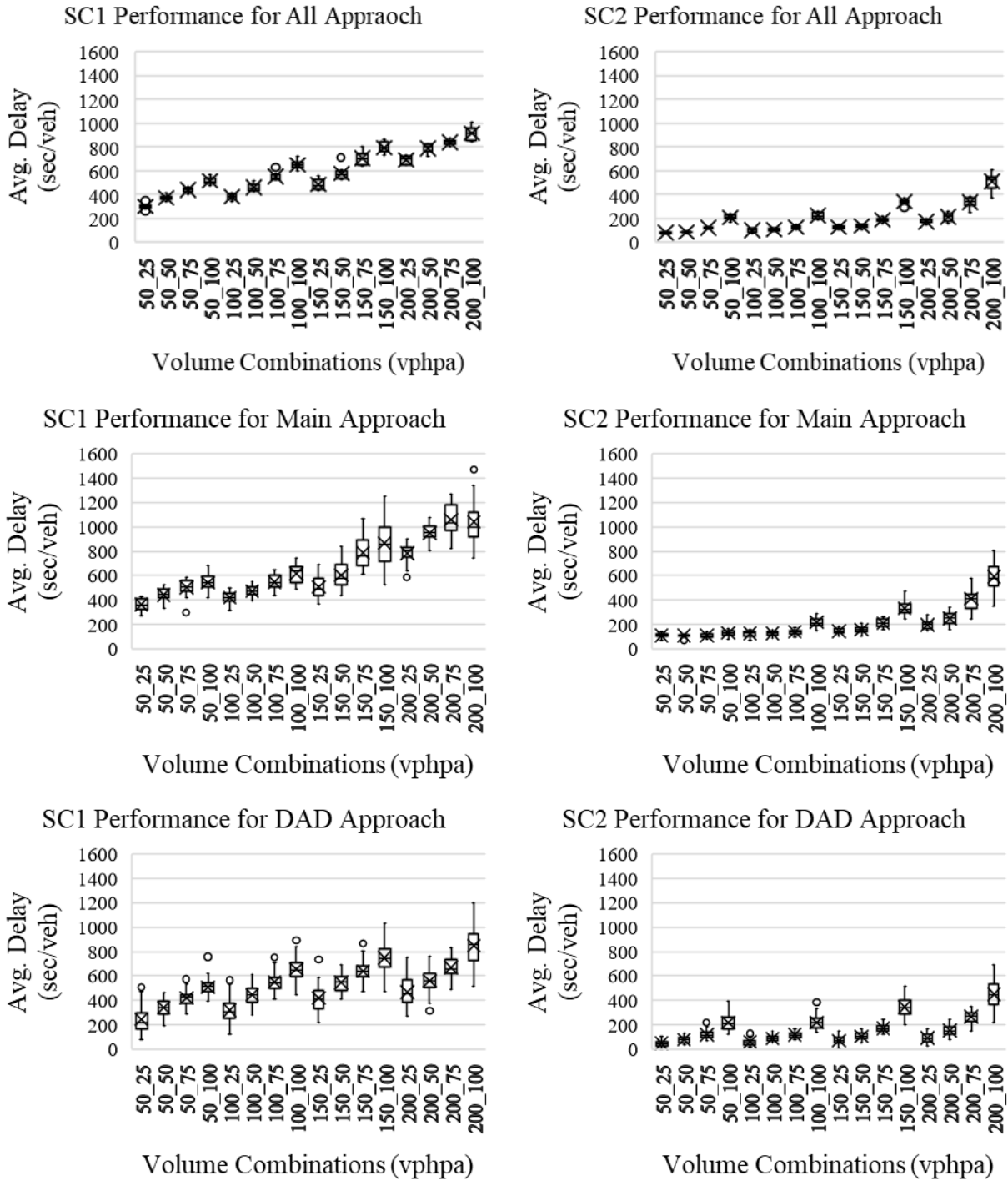
Figure C.1 Average delay for All, Main and DAD approach under SC1 and SC2 for DAD approach volume increase for various levels of constant Main approach volume (WZL=1.1 mile, N_{DAD}=5 , T_{M\%}=20 , T_{DAD\%}=5 )
