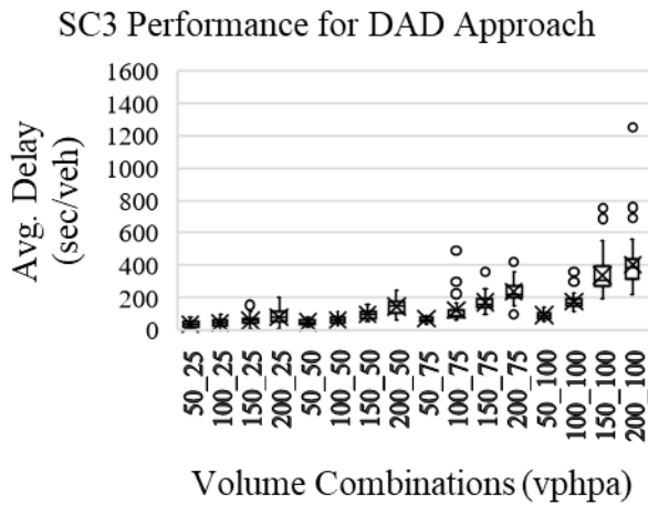
Figure C.4 Average delay for All, Main and DAD approach under SC3 and SC4 for Main approach volume increase for various levels of constant DAD approach volume (WZL=1.1 mile, N_{DAD}=5 , T_{M\%}=20 , T_{DAD\%}=5 )
