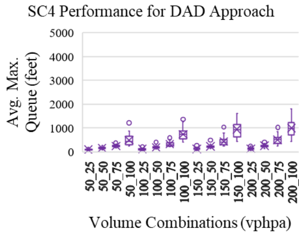
Figure C.6 Average maximum queue for All, Main and DAD approach under SC3 and SC4 for DAD approach volume increase for various levels of constant Main approach volume (WZL=1.1 mile, N_{DAD}=5 , T_{M\%}=20 , T_{DAD\%}=5 )
