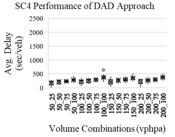
Figure B.2 Average delay for All, Main and DAD approach under SC3 and SC4 for DAD approach volume increase for various levels of constant Main approach volume (WZL=1.1 mile, N_{DAD}=3 , T_{M\%}=20 , T_{DAD\%}=5 )
