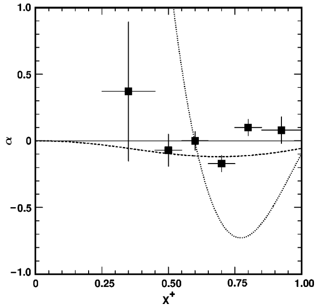
FIG. 6. The values of \alpha for each momentum bin are represented by the solid squares. Errors shown are the statistical and systematic errors added in quadrature. The solid line represents the statistical model. The dotted line represents the function predicted by Suzuki [23]. The dashed line is the function of Cheung and Yuan [24].
