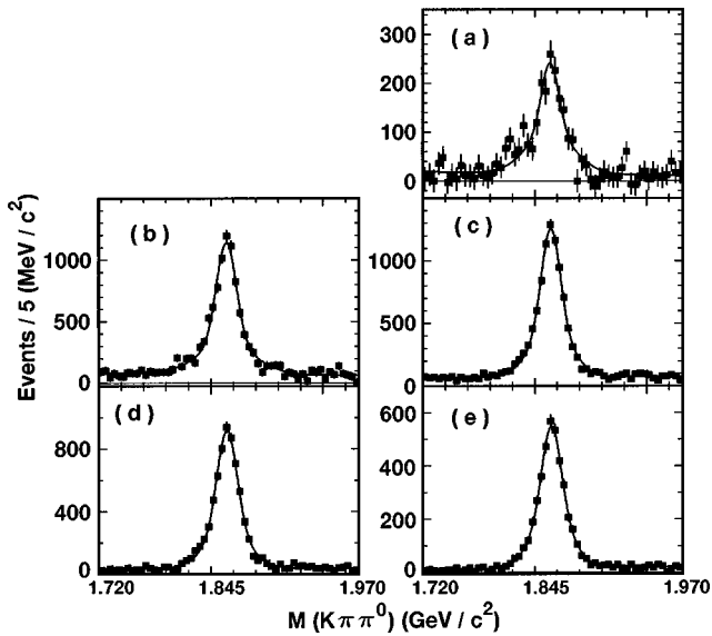
FIG. 4. M(K\pi\pi^0) after sideband subtraction for the five x^+ ranges (a) 0.45 < x^+ < 0.55 , (b) 0.55 < x^+ < 0.65 , (c) 0.65 < x^+ < 0.75 , (d) 0.75 < x^+ < 0.85 , (e) 0.85 < x^+ < 1.0 . The solid squares are the data points and the solid line is the fitting function as described in Sec. IV.
