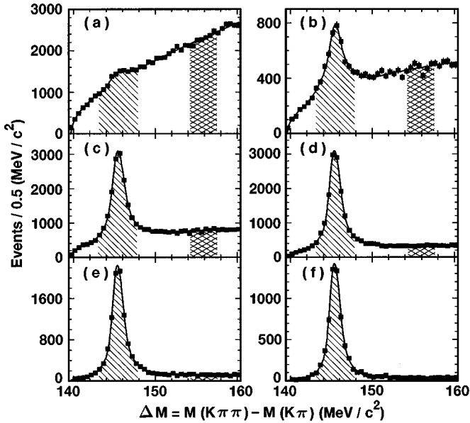
FIG. 1. D^* - D mass difference for the D^0 \rightarrow K\pi decay mode for the six x^+ ranges (a) 0.25 < x^+ < 0.45 , (b) 0.45 < x^+ < 0.55 , (c) 0.55 < x^+ < 0.65 , (d) 0.65 < x^+ < 0.75 , (e) 0.75 < x^+ < 0.85 , (f) 0.85 < x^+ < 1.0 . The solid squares are the data points and the solid line is the fitting function as described in Sec. IV. The hatched area is the signal region while the crosshatched region is the sideband.
