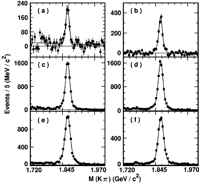
FIG. 3. M(K\pi) after sideband subtraction for the six x^+ ranges (a) 0.25 < x^+ < 0.45 , (b) 0.45 < x^+ < 0.55 , (c) 0.55 < x^+ < 0.65 , (d) 0.65 < x^+ < 0.75 , (e) 0.75 < x^+ < 0.85 , (f) 0.85 < x^+ < 1.0 . The solid squares are the data points and the solid line is the fitting function as described in Sec. IV.
