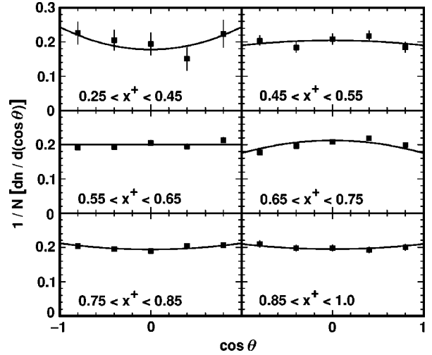
FIG. 5. Normalized \cos \theta distributions in the six x^+ ranges for the D^0 \rightarrow K^- \pi^+ and D^0 \rightarrow K^- \pi^+ \pi^0 decay modes combined. The solid squares are the efficiency-corrected yields for each \cos \theta bin in the specified x^+ range. These distributions are fit with the function W(\cos \theta) = 0.4N(1 + \alpha \cos^2 \theta) , where the factor of 0.4 is the bin width and N = 3/(6 + 2\alpha) .
