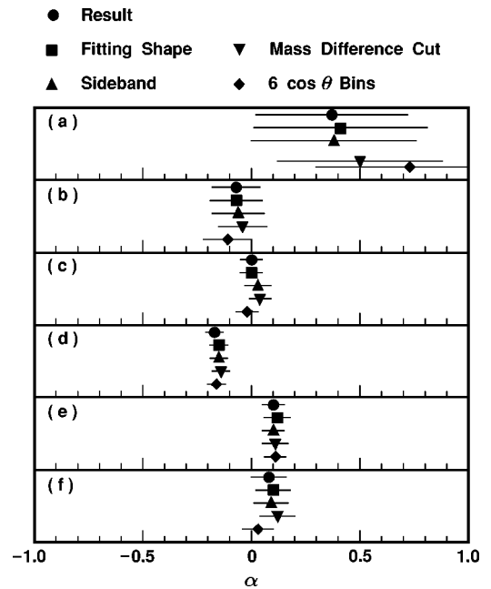
FIG. 7. The results from the systematic error studies for the six x^+ bins (a) 0.25 < x^+ < 0.45 , (b) 0.45 < x^+ < 0.55 , (c) 0.55 < x^+ < 0.65 , (d) 0.65 < x^+ < 0.75 , (e) 0.75 < x^+ < 0.85 , (f) 0.85 < x^+ < 1.0 . The different symbols represent the resulting values of \alpha using the modifications in the analysis procedure as described in Sec. VII.
