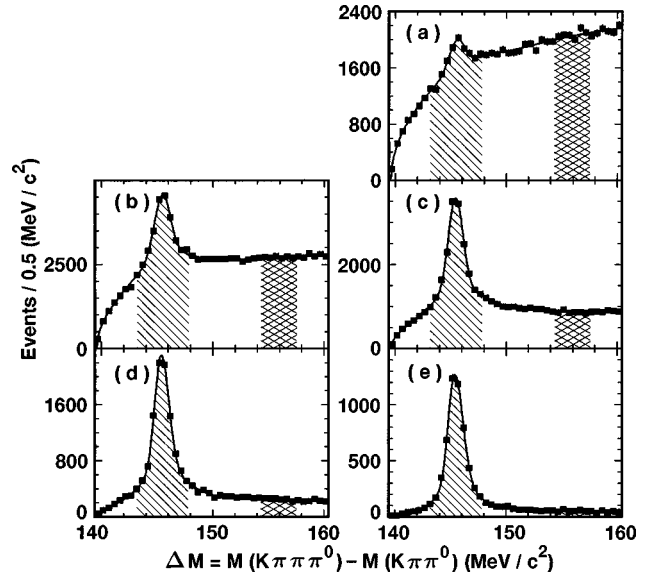
FIG. 2. D^* - D mass difference for the D^0 \rightarrow K\pi\pi^0 decay mode for the five x^+ ranges (a) 0.45 < x^+ < 0.55 , (b) 0.55 < x^+ < 0.65 , (c) 0.65 < x^+ < 0.75 , (d) 0.75 < x^+ < 0.85 , (e) 0.85 < x^+ < 1.0 . The solid squares are the data points and the solid line is the fitting function as described in Sec. IV. The hatched area is the signal region while the crosshatched region is the sideband.
