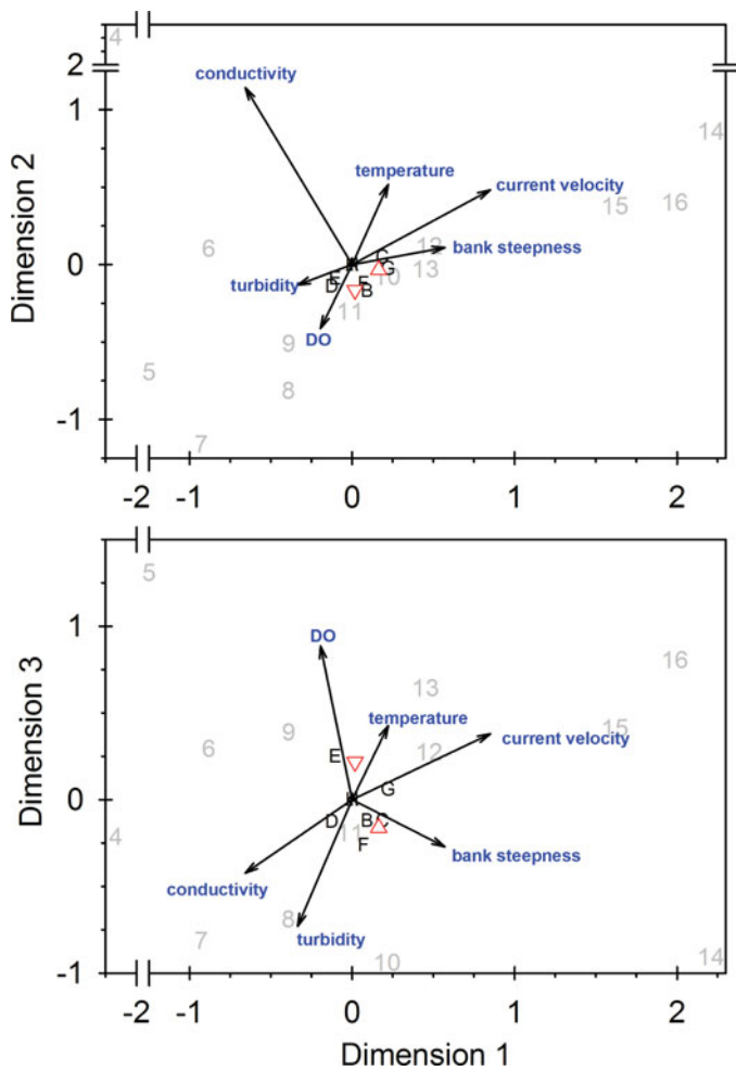
FIGURE 5. Canonical correspondence analysis ordination diagram of the first three canonical dimensions for the 13 stations where bank habitat was sampled by boat-mounted electrofisher in the lower Rio Grande, January-March 2006. Arrows indicate the environmental variables, and arrowheads indicate the increase in gradient. Numbers represent the study reaches, and letters represent the centroids for the nine most abundant species as listed in Table 1. The centroids for Common Snook are represented by open triangles with downward pointing triangles representing age-1 fish and upwards pointing triangles representing age-2 fish.
