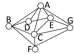
Figure 2: Primal graph.
