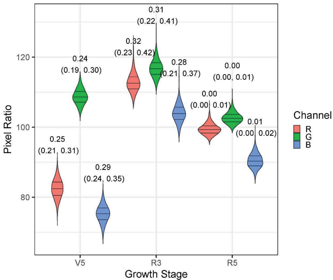
Figure 25. Red green and blue digital image channels relationship with growth stage at time of phenotyping and broad sense heritability and 95% confidence intervals on an entry mean basis during 2017-2018 water response experiment across populations, environments, and irrigation treatments
