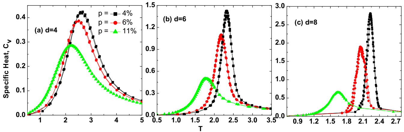
FIG. 3. Specific heat C vs dimensionless temperature T for (3,4) QHP models with distances (a) d = 4 , (b) d = 6 , and (c) d = 8 , at p values as indicated on panel (a). Each curve contains data points from the feedback-optimized parallel tempering simulation where ordered and disordered configurations are used as initial states. The peak positions are extrapolated to infinite distance to obtain the transition temperatures (see Fig. 5).
