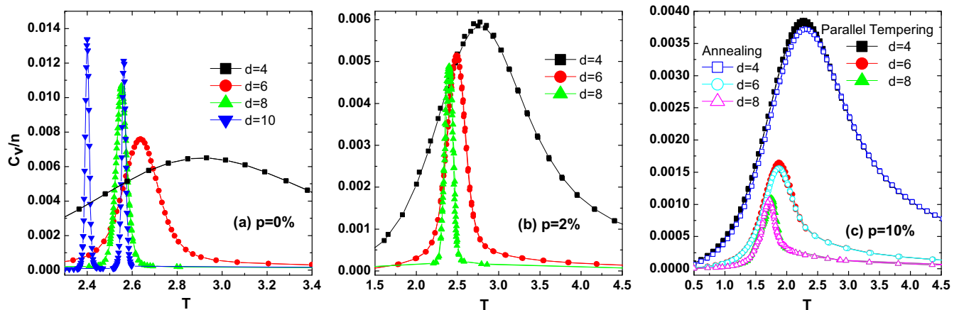
FIG. 4. Specific heat C divided by the number of bonds n vs dimensionless temperature T for (3,4) QHP models at (a) p = 0 , (b) p = 2\% , and (c) p = 10\% , with code distances as indicated in the captions. Each curve contains data points from the feedback-optimized parallel tempering simulation. The annealing plot contains data points from upward and downward temperature sweeps. Relatively weak variation of the peak height with system size is indicative of a discontinuous transition. Open symbols in plot (c) show the data obtained with annealing, which agrees with the parallel tempering data (filled symbols).
