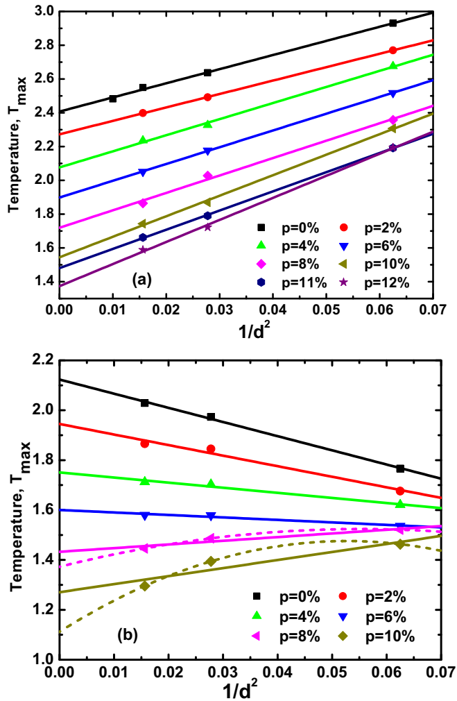
FIG. 5. (a) Finite-size scaling of the dimensionless temperatures T_{\max} where specific heat reaches the maximum for (3,4) QHP models vs the inverse square of the code distance, with the fraction of flipped bonds p as indicated. For the point p = 0 and d = 10 where we could not eliminate the hysteresis, the average temperature was used. (b) The same for the dual (3,4) QHP models. To accommodate the increased curvature, for p = 0.08 and 0.10 we also used parabolic fits, T_{\max} = T_c + A/d^2 + B/d^4 , which results in a significantly reduced extrapolated value of T_c for p = 0.10 . The T_c values from parabolic fits are shown in Fig. 1 with open red symbols.
