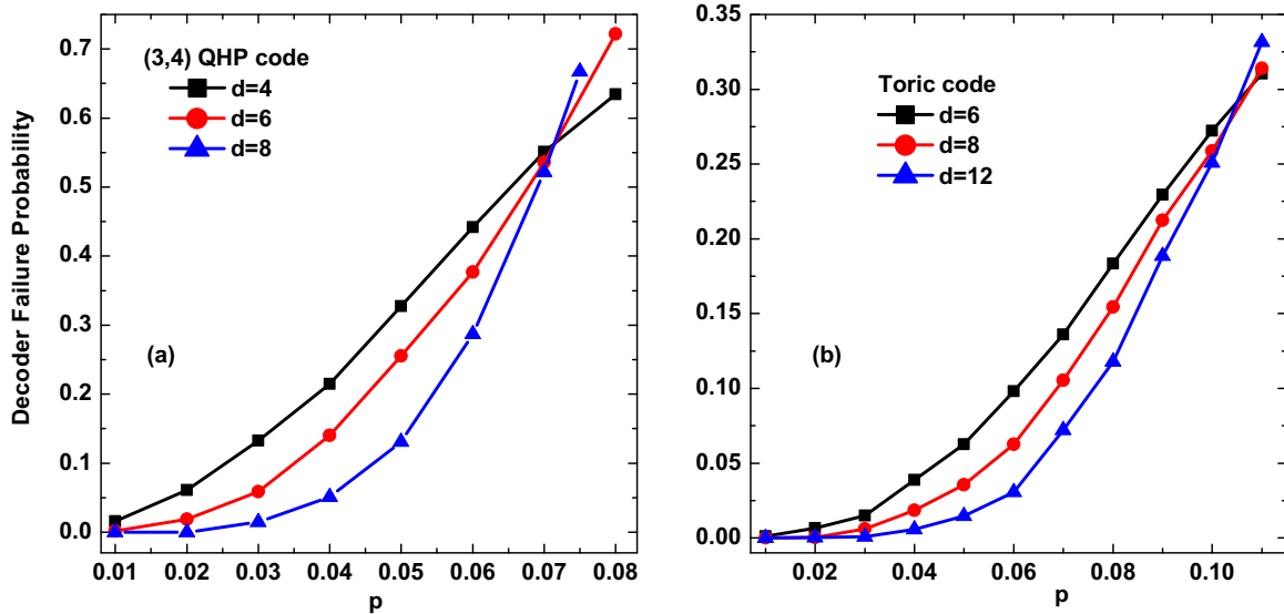
FIG. 2. Decoder failure probability as a function of bit-flip error probability for three (3,4) QHP codes (left) and the rotated toric codes (right). The decoding was performed over 1024 error realizations for (3,4) QHP codes and over 4096 error realizations for toric codes. The corresponding decoding pseudthreshold is close to p = 7.0\% for (3,4) QHP codes and to 10.4\% for toric codes.
