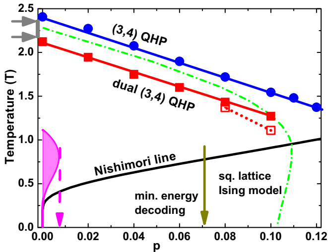
FIG. 1. The (p, T) phase diagram of the two random-bond Ising models associated with QHP codes from a (3,4) Gallager ensemble, labeled “(3,4) QHP” and “dual (3,4) QHP,” where the latter model includes a summation over additional spin variables corresponding to the codewords, see Eq. (5). Here p is the error probability and T the dimensionless temperature. Positions of the specific heat maxima at different p , extrapolated to infinite system size, are shown with solid blue circles and solid red boxes with ad hoc linear fits [red open boxes connected with a dotted line correspond to parabolic extrapolation in Fig. 5(b)]. The two transition lines intersect the p = 0 axis in approximately mutually dual temperatures and are located, respectively, above and below the critical temperature for the square-lattice random-bond Ising model (dashed-dotted green line; data from Ref. [33]). The ML decoding problem corresponds to the points on the Nishimori line shown with a solid black line; a temperature not on the Nishimori line corresponds to a suboptimal decoder which assumes an incorrect error probability. The magenta-shaded region shows the lower bound for the decodable region from Theorem 2; the rightmost point of this region coincides with the lower bound obtained by analyzing minimum-energy decoder in Ref. [16] (dashed magenta downward arrow). The forest-green solid vertical arrow shows our numerical estimate for the minimum-weight decoding threshold, see Sec. IV B. The temperatures T_{\max} and its dual, T_{\max}^* from Theorem 3, are marked with a pair of horizontal arrows separated by a gray bar on the vertical axis; the lower arrow corresponds to the analytical upper temperature bound of the decodable region. A more accurate upper bound from the present data is given by the “dual (3,4) QHP” line.
