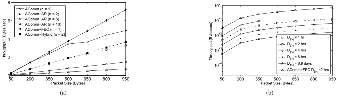
Fig. 5. Throughput results: (a) T_{life} = 5 years using AComm protocols and (b) Using HComm-Hybrid with q = 2.5 mobile nodes per 100 UG nodes.
