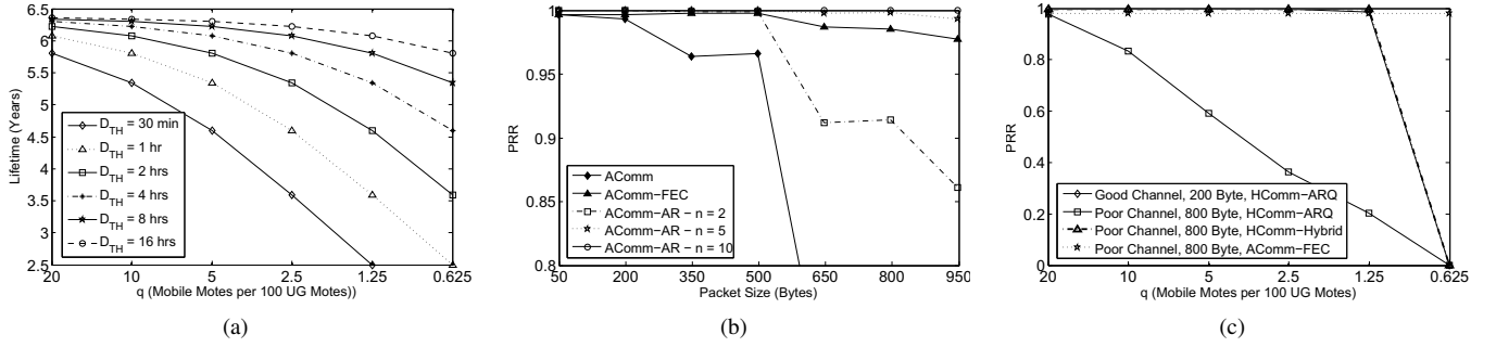
Fig. 4. (a) Network lifetime in terms of q and D_{TH} for AComm and AComm-FEC, (b) PRR of the announcement protocols in good channel conditions, (c) PRR using HComm-ARQ and HComm-Hybrid (FEC) in various conditions and packet sizes with D_{TH} = 2 hours.
