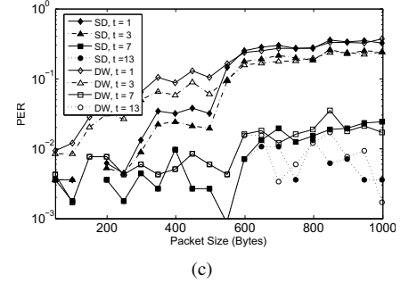
Fig. 2. (a) Pictures of the experiments, (b) Average attempts (ARQ) and bits in error (FEC), and (c) PER of various FEC encryption strengths.
