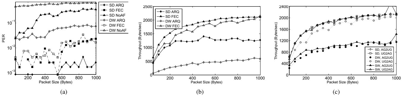
Fig. 3. (a)PER of various error control protocols, (b) UG2AG throughput in good (SD) and poor (DW) conditions using ARQ ( n = 5 ) and FEC ( t = 7 ), (c) Throughput vs. packet size for SD, SW, and DW.
