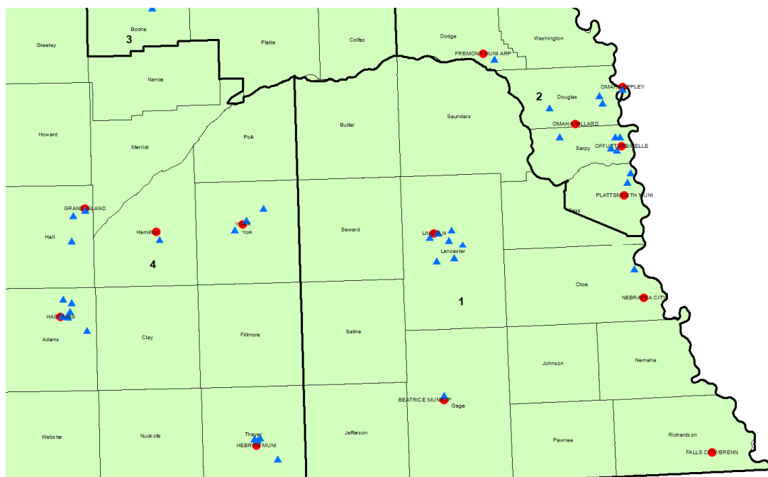
Figure 3.2. Southeast Nebraska counties with four Nebraska Department of Transportation (NDOT) maintenance districts visible outlined in the thick black line. The red dots indicate Automated Surface Observing System (ASOS) stations. The blue triangles show Global Historical Climate Network-Daily (GHCN-D) sites within approximately 9 mi. (15 km) of the ASOS stations that had sufficient data for the analysis.
