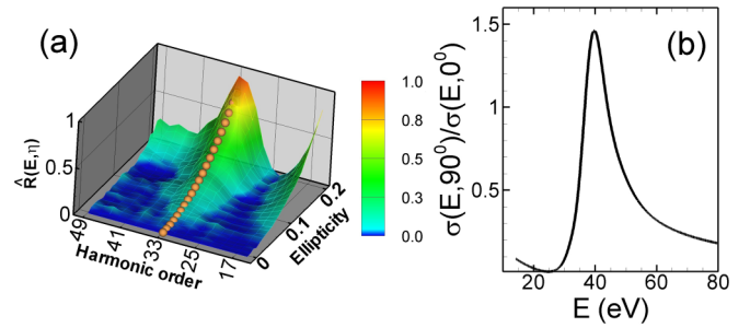
FIG. 2. (a) Experimental results for \hat{R}(E, \eta) [see Eq. (8)] as a function of harmonic order N and ellipticity \eta . Yellow spheres mark the 33rd harmonic. (b) The ratio \sigma(E, 90^\circ)/\sigma(E, 0^\circ) = [1 - \beta(E)/2]/[1 + \beta(E)] [cf. Eq. (2)] as a function of the photoelectron energy E [obtained from theoretical random-phase approximation with exchange (RPAE) results for \beta(E) [32]].
