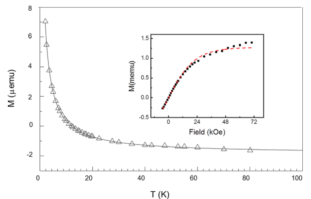
FIG. 3. ZFC measurement of Cu(Fe) clusters embedded in a \text{SiO}_2 matrix. The solid line is the fit to the data. The inset is the M vs. H curve measured at 2 K and the dashed line is the Brillouin function fit to the data.
