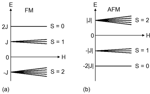
FIG. 4. Energy levels for two interacting S = 1 atoms with (a) ferromagnetic and (b) AFM RKKY interaction.
