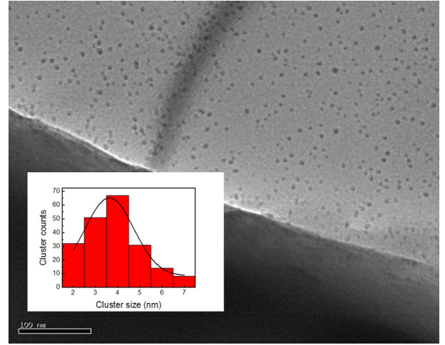
FIG. 2. TEM image of Cu(Fe) clusters deposited on TEM grid. The inset is the cluster size distribution measured from the sample.
