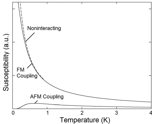
FIG. 5. Susceptibility of non-interacting and interacting Fe atoms in Cu. Only pairs of Fe atoms interacting by positive or negative RKKY interactions are considered, and the susceptibility of the non-interacting system has been normalized to agree with the high-temperature part of the FM curve.
