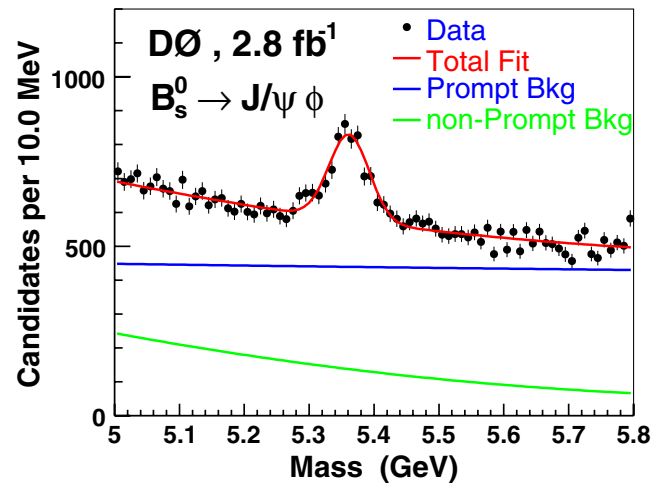
FIG. 1 (color online). The invariant mass distribution of the ( J/\psi , \phi ) system for B_s^0 candidates. The curves are projections of the maximum likelihood fit (see text).
