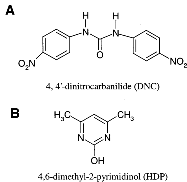
Figure 1. Structures of 4,4'-dinitrocarbanilide (DNC) and 4,6-dimethyl-2-pyrimidinol (HDP), the ingredients in Nicarbazine.
