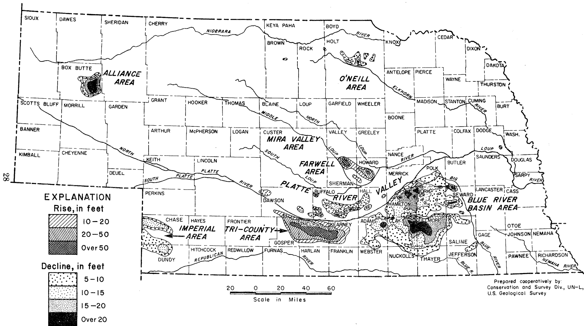
Figure 8.--Principal areas in Nebraska where groundwater levels for the fall of 1973 show a significant rise or decline from assumed normal water level.
