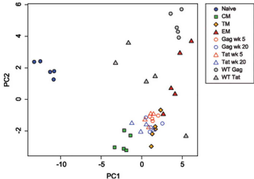
Fig 4. Principal component analysis of transcription factor expression profiles from SIV-specific MHC tetramer-sorted CD8 + T cells from animals vaccinated with SIV \Delta nef, animals infected with wild-type SIV, and sorted CD8 + T cell subsets. Plot of principal components 1 and 2 for each of the expression profiles assessed from sorted naïve and memory CD8 + T cell subsets, SIV-specific MHC tetramer-sorted CD8 + T cells isolated from SIV \Delta nef-vaccinated animals, and MHC tetramer-sorted CD8 + T cells isolated from animals (n = 5) at 20 weeks following wild-type SIV infection. Principal components 1 and 2 explain 77 percent of cumulative total variance.
