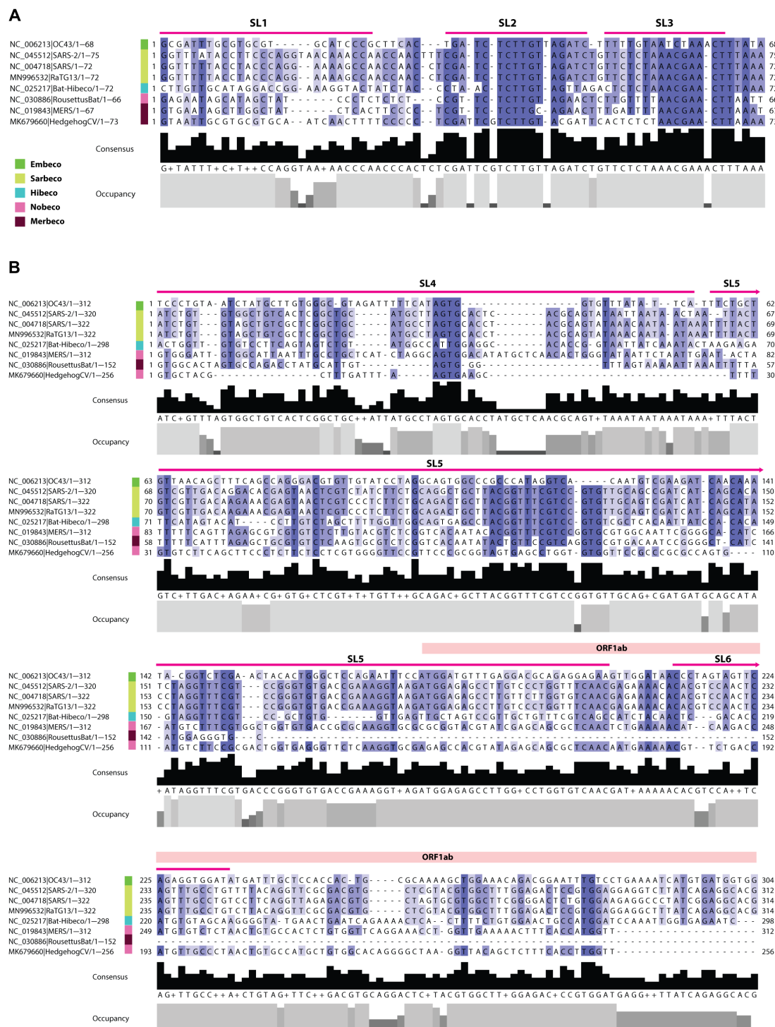
Fig. 3. Conservation of 5'-end sequences encoding RNA structures in betacoronavirus genomes. Multiple sequence alignment showing percentage identity and sequence coverage within the 5'-UTR and adjacent region of representative species within genus Betacoronavirus . (A) SL1–3. (B) SL4–6. Viral subgenus is indicated as shown in the key. Sequence numbering is standardized to the genome sequence start position of each taxon. Taxon labels show GenBank accession numbers and abbreviated virus names. OC43, human coronavirus OC43; RousettusBat, Rousettus bat coronavirus; MERS, Middle East respiratory syndrome–related coronavirus; Bat-Hibeco, Bat Hp-betacoronavirus.
