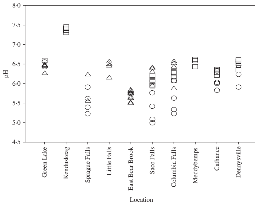
FIG. 2. Stream pH measurement collected at eastern Maine, study sites at which Salmo salar smolts were held in 2004 (□), 2005 (○) and 2006 (△).
