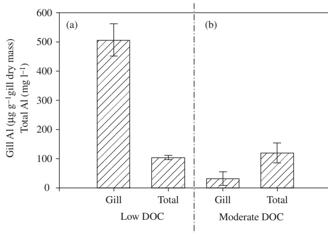
FIG. 6. Comparison of Salmo salar smolt gill aluminium after 72 h exposures to (a) East Bear Brook, eastern Maine, with low dissolved organic carbon (DOC) stream water and to (b) other eastern Maine study sites with similar pH and similar levels of total water aluminium but moderate DOC. A 40% mortality rate of S. salar smolts was observed under the conditions present at East Bear Brook, whereas no mortality was observed at the other sites. Values are the means \pm s.d. of three exposure periods at East Bear Brook and five exposure periods at the other sites consisting of at least 12 fish per exposure.
