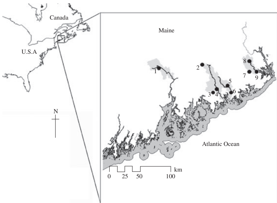
FIG. 1. Locations of catchments (□) and specific sites (●) used during the streamside study in eastern Maine, U.S.A., from 2004 to 2006. —, selected historic Salmo salar rivers; 1, Kenduskeag; 2, East Bear Brook; 3, Spragues Falls; 4, Little Falls; 5, Saco Falls; 6, Columbia Falls; 7, Cathance; 8, Meddybemps; 9, Dennysville.
