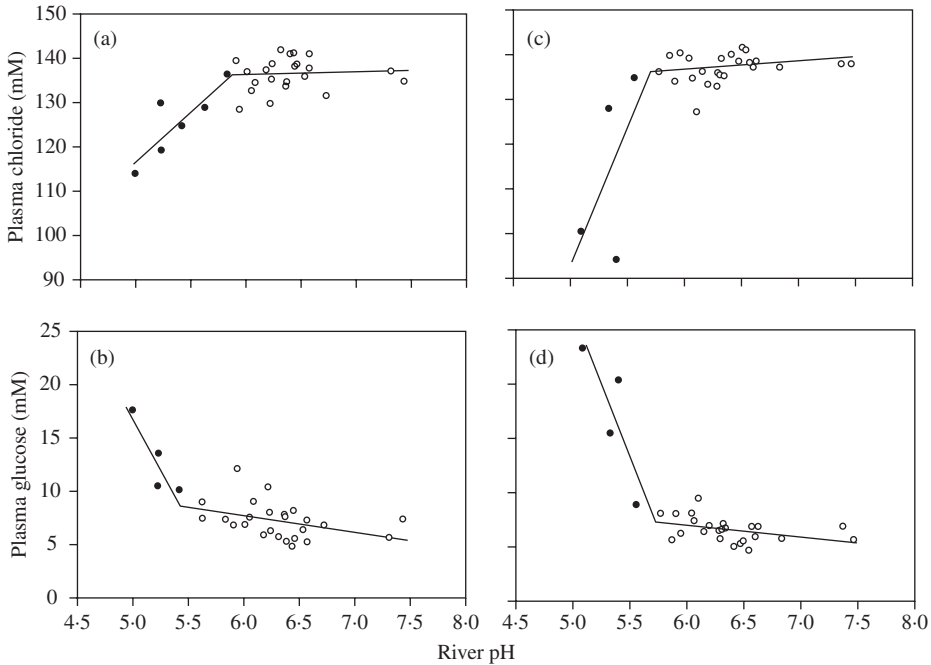
FIG. 3. Physiological response in (a), (c) plasma chloride and (b), (d) plasma glucose of Salmo salar smolts exposed to ambient water chemistry conditions at various study sites throughout eastern Maine, for (a), (b) physiological response of S. salar smolts after a 3 day and (c), (d) 6 day exposure to ambient stream pH. The estimated changepoint (○) or break point (●) in physiological response of S. salar smolts to stream pH are illustrated. Each point is the mean of 12 individuals sampled from two replicate tanks (see Table III).
