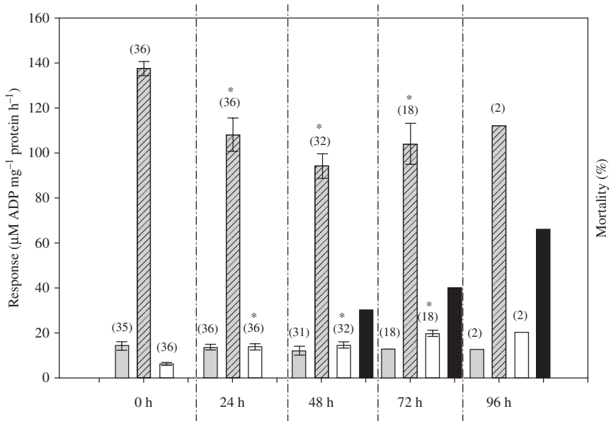
FIG. 4. Physiological response of Salmo salar smolts exposed to ambient water chemistry conditions at East Bear Brook, eastern Maine, during spring 2006: Na + - and K + -ATPase ( \mu\text{M ADP mg}^{-1} \text{ protein h}^{-1} ) ( \square ), plasma chloride ( \square ) and plasma glucose ( \square ) and mortality (%) ( \blacksquare ). Values are mean \pm s.d. Sample size is given in parentheses above each bar. *, a significant statistical difference ( P < 0.05 ) when compared with 0 h.
