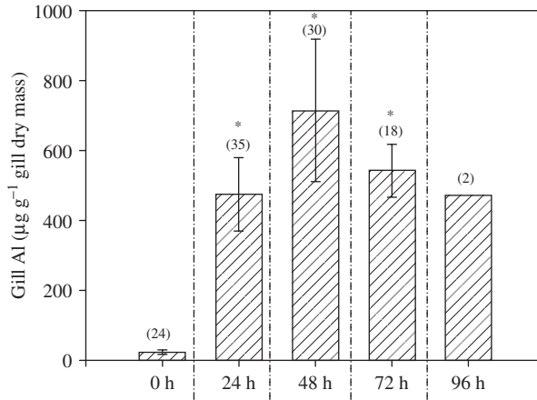
FIG. 5. Gill aluminium concentrations of Salmo salar smolts exposed to ambient conditions at East Bear Brook, eastern Maine, during the 2006. Values are mean \pm s.d. Sample size is given in parentheses above each bar. *, a significant statistical difference ( P < 0.05 ) when compared with 0 h.
