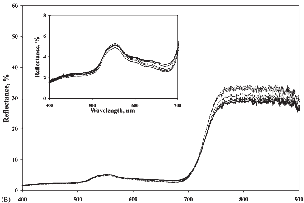
Figure 2. Summary of canopy reflectances acquired by (A) hand-held sensors and (B) boom-held sensors.
