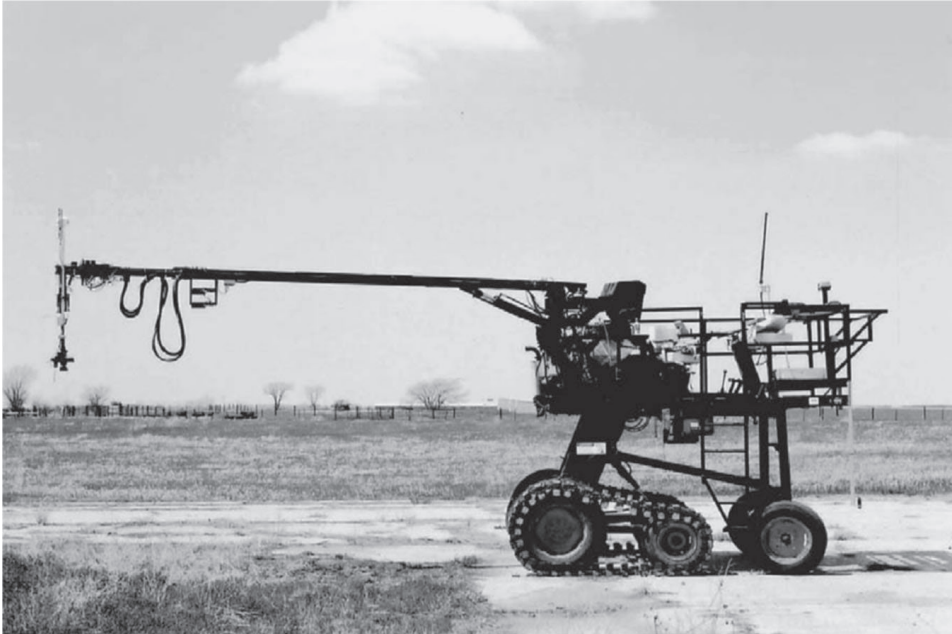
Figure 1. The Goliath platform.
