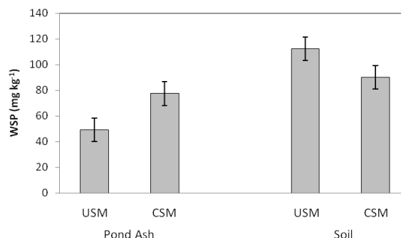
Figure 3. Water-soluble phosphorus (WSP) content as affected by unconsolidated surface material (USM) and consolidated subsurface material (CSM) for the pond ash amended surfaces and soil surfaces. Values for WSP content are averages from four plots. Vertical bars are standard errors.
