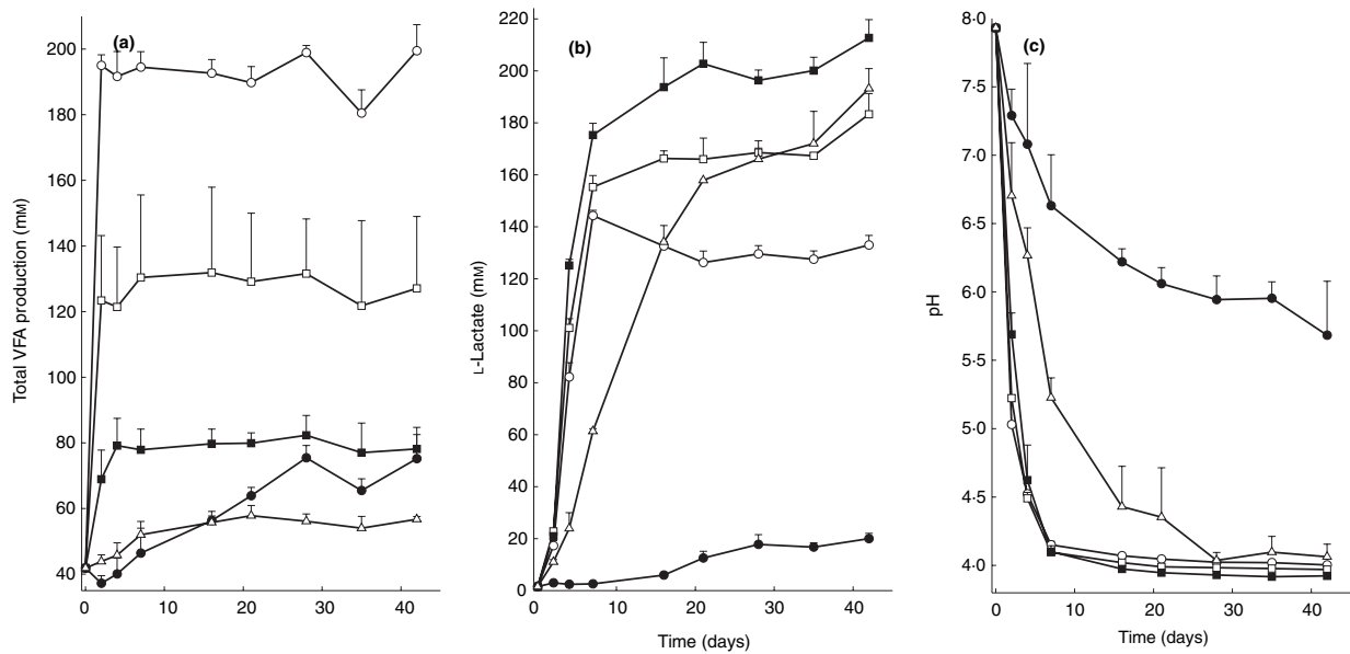
Fig. 1 Effect of thymol and eugenol treatments on VFA, lactate and pH in stored cattle waste. Treatments included: ○ control (no additions); ● thymol 13.4 mM; □ eugenol 10.05 mM; ■ eugenol 13.4 mM and △ eugenol 16.75 mM
