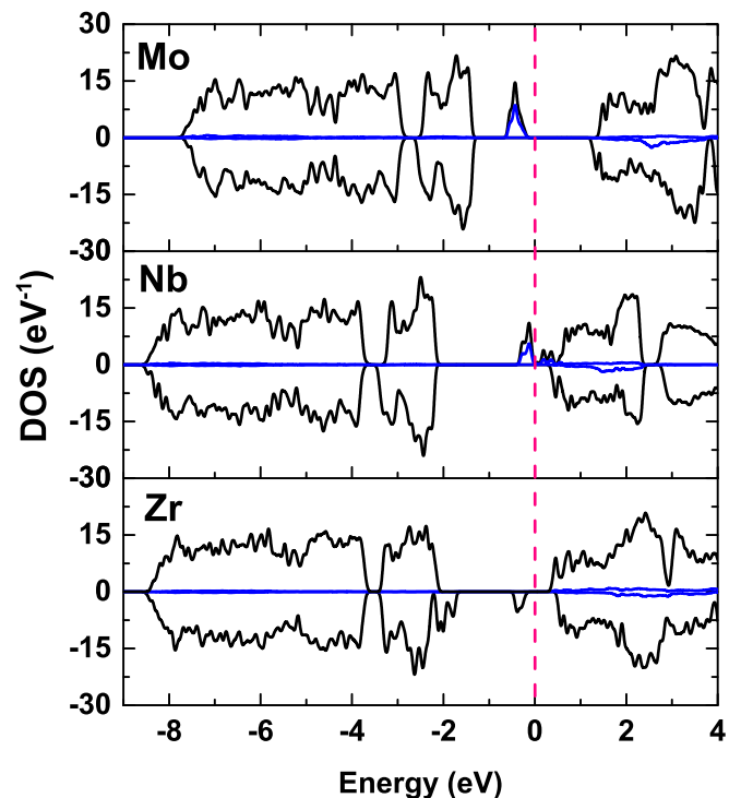
FIG. 9. Total density of states (DOS) of Zr, Nb, and Mo doped \text{Cr}_2\text{O}_3 , shown in black lines. The 4d impurity states are shown in blue lines. \pm sign of DOS indicates different spin channels. The Fermi energy has been shifted to 0 \text{ eV} .
