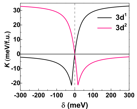
FIG. 8. MCA as a function of the t_{2g} crystal-field parameter \delta , at \xi = 35 meV, for 3d^1 and 3d^2 configurations. Note the different scale (meV) for MCA compared to Fig. 5.
