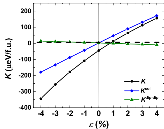
FIG. 2. Dependence of K (black circles) and K_{\text{col}} (blue diamonds) on the in-plane strain under biaxial stress in \text{Cr}_2\text{O}_3 . Green triangles: Dipole-dipole contribution to MAE. Dashed line: Experimental MAE of unstrained \text{Cr}_2\text{O}_3 .
