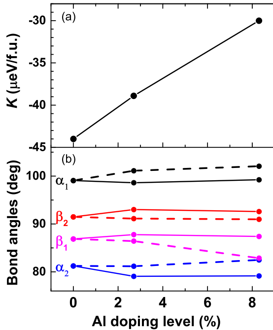
FIG. 6. Effect of Al doping on (a) K and (b) O-Cr-O bond angles defined in Fig. 1. Solid and dashed lines in (b) correspond to Cr atoms that are, respectively, first- and second-nearest neighbors of Al. For the latter, the angles are averaged over the triplets of bonds that are equivalent in pure \text{Cr}_2\text{O}_3 .
