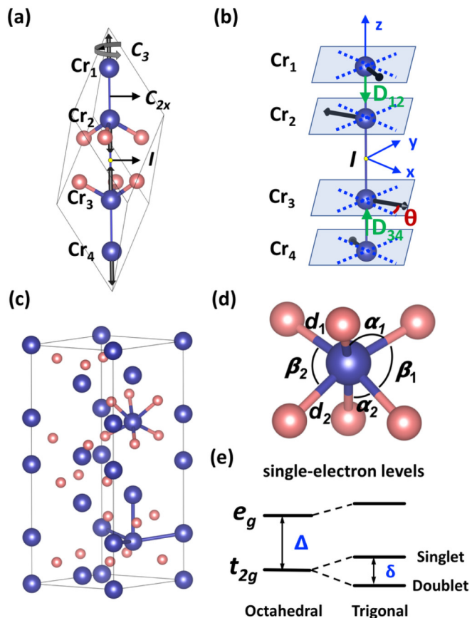
FIG. 1. (a) Rhombohedral primitive and (c) hexagonal unit cell of \text{Cr}_2\text{O}_3 . Blue (red) spheres denote Cr (O) atoms. Here we denote the threefold rotation axis (rhombohedral axis or hexagonal axis) as the z axis. The symmetry operations of paramagnetic \text{Cr}_2\text{O}_3 (inversion center I , threefold rotation axis C_3 , and twofold rotation C_{2x} ) are labeled in (a). Black arrows attached to Cr atoms denote their spin orientations. (b) Spin canting arising when the primary AFM order parameter \mathbf{L} is along the x axis. Green arrows show the DMI vectors. (d) Local environment of the Cr atom showing bond angles and lengths. (e) Single-electron energy levels and crystal-field splitting parameters ( \Delta , \delta ). Structure visualization is done using VESTA [9].
