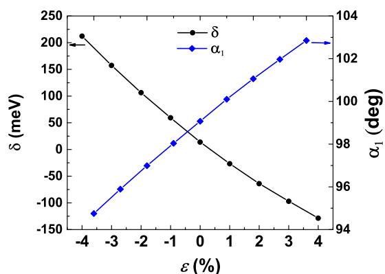
FIG. 4. Epitaxial strain-dependent t_{2g} level splitting \delta and the O-Cr-O bonding angle \alpha_1 .
