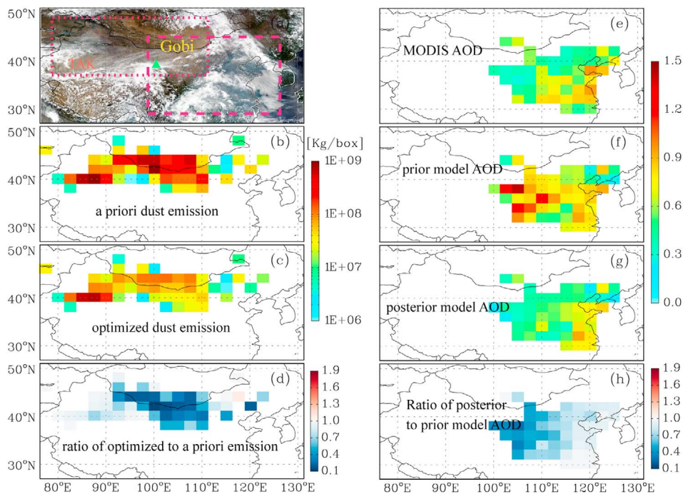
Figure 1. (a) True color image from MODIS/Aqua on 27 May 2008. The region within the rectangle of dashed line is the downwind plume region where the observational data are used. The region within the rectangle of dotted line is used for validation. (b) The prior mineral dust emission for the period of 25–28 May 2008. (c) Same as Figure 1b but for optimized dust emission. (d) The ratio of the optimized to prior dust emission. (e) MODIS AOD at 0.67 \mu\text{m} aggregated to GEOS grid box and averaged for the period of 25–28 May 2008, which served as observational constraint for the adjoint inverse modeling of dust emission. (f) GEOS-chem total AOD at 0.67 \mu\text{m} simulated with prior dust emission averaged over satellite overpass time period (see text for details). (g) Same as Figure 1f but for the AOD simulated with optimized emission. (h) Ratio between Figures 1f and 1g.
