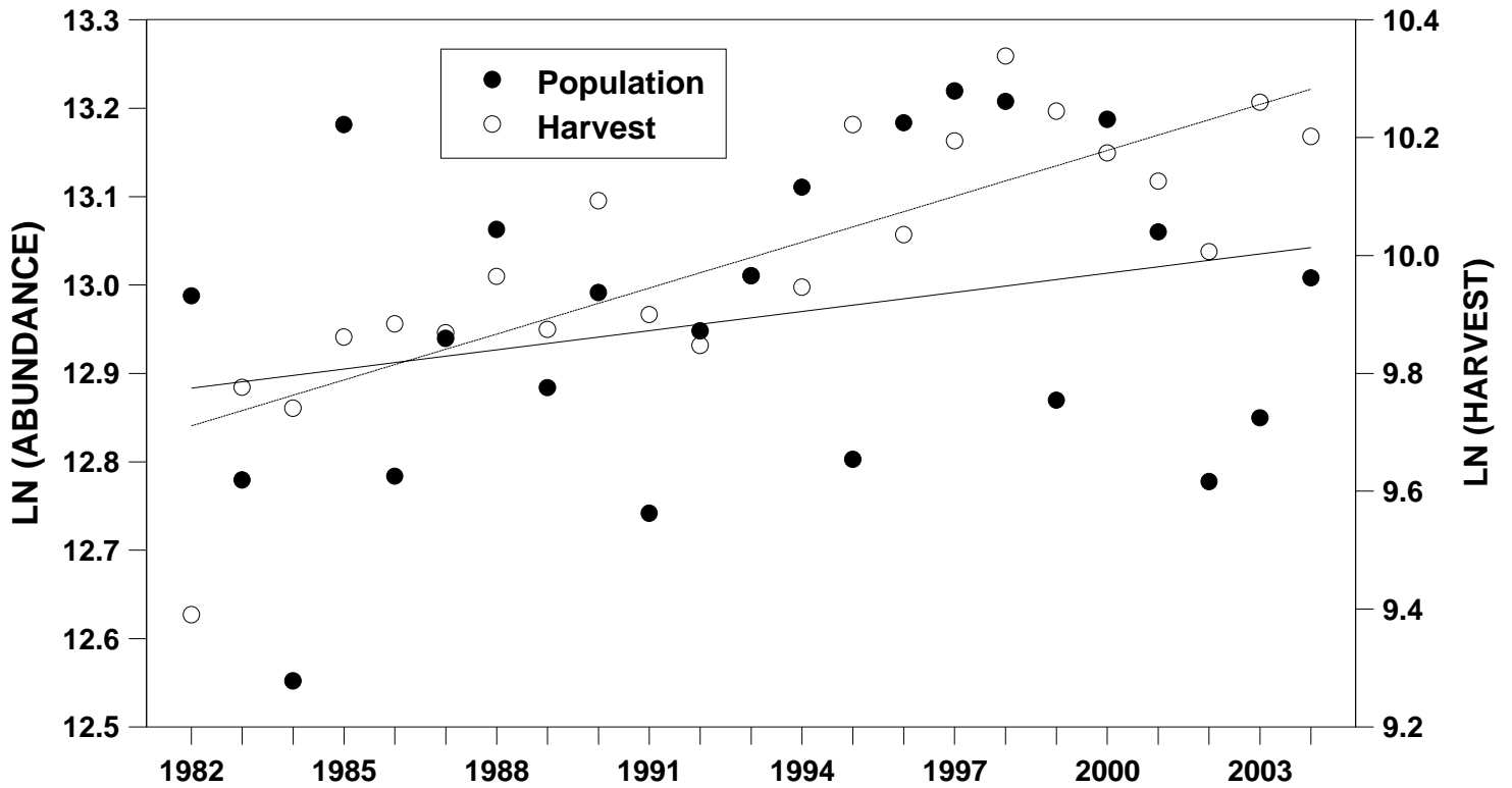
Figure 14. Trend analyses of indices to abundance and harvest of Mid-Centinet sandhill cranes
