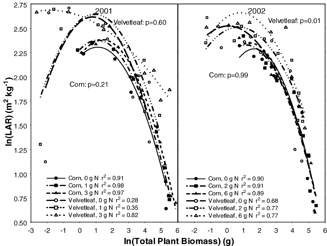
FIGURE 3. Natural log of leaf area ratio (LAR, \text{m}^2 \text{ leaf kg}^{-1} total plant biomass) plotted as a function of natural log of total plant biomass in 2001 and 2002. Curves represent best-fit second order polynomial regressions, and r^2 values indicate goodness of fit. Probability values for each species correspond to the test that leaf area ratio did not differ across nitrogen treatments.
