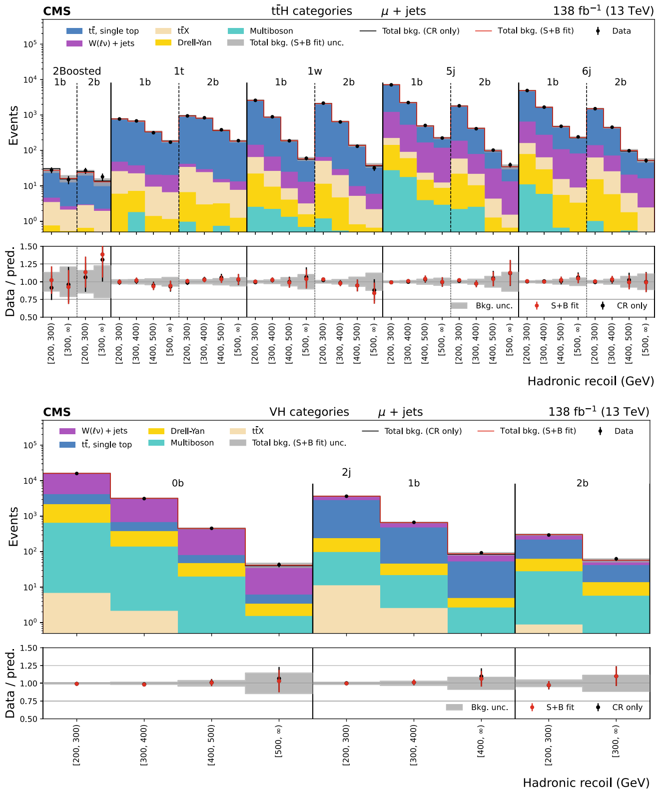
Fig. 2 Distributions of hadronic recoil in the \bar{t}\bar{t}H (upper plot) and VH (lower plot) categories for the \mu + \text{jets} CR. The black histogram shows the total background (bkg.) prediction from a CR only, B-only fit, while
