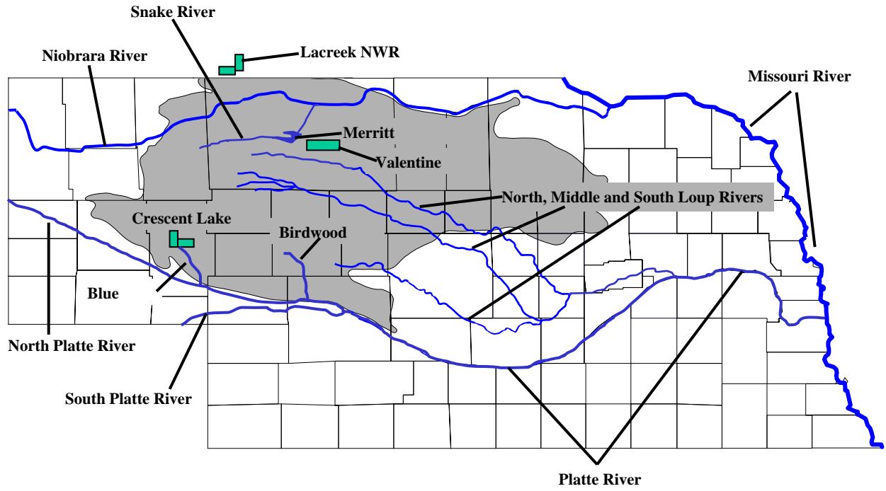
Figure 1. Location of the Sandhills of Nebraska (shaded portion), Lacreek National Wildlife Refuge, and important wintering locations of trumpeter swans.
