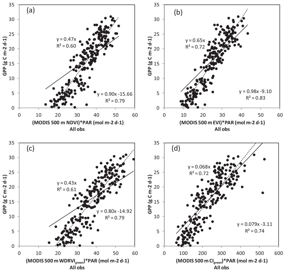
Fig. 1. Relationships between VI \times (daily PAR) vs. tower flux daily GPP for the US-NE1 site: (1) NDVI \times PAR vs. GPP; (2) EVI \times PAR vs. GPP; (3) WDRVI green \times PAR vs. GPP; and (4) CI green \times PAR vs. GPP. The solid lines force intercepts to zero (upper eqns.) while dashed lines do not (lower eqns.). All observations are included.
