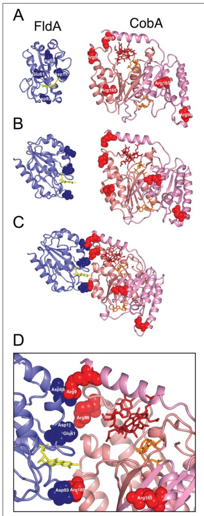
FIGURE 2. Computer model of the CobA-FldA complex. A , crystal structures of CobA (monomers are colored salmon and pink) and FldA (light blue) are shown. Selected basic surface residues on FldA are colored blue, whereas selected acidic side chains on CobA are colored red. B , the structures in A are rotated 90° toward each other. C , CobA and FldA
