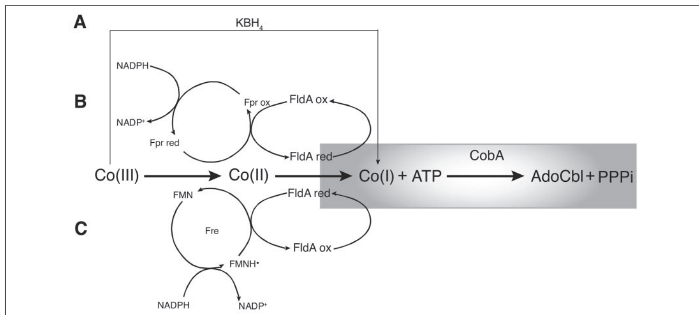
FIGURE 1. Assays used to assess the production of AdoCbl by CobA. A, \text{KBH}_4 is used to reduce Co(III)Cbl to Co(I)Cbl directly. B, the Fpr/FldA system converts cob(III)alamin to cob(I)alamin. CobA (represented by the shaded box) binds cob(II)alamin and Mg/ATP. Reduced FldA then provides the electron to reduce cob(II)alamin in the CobA active site. C, in these studies we attempted to bypass Fpr by providing reduced flavins using Fre and NADPH.
