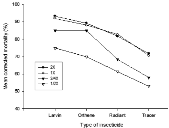
Fig. 2. Percent mortality of fall armyworm (FAW) third instar larvae caused by different rates of various insecticides.
