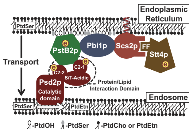
FIGURE 8. A model of the PstB transport complex. We propose that the PstB lipid transfer event is facilitated by a complex of proteins on the acceptor membrane consisting minimally of PstB2p and PstB2p. We further hypothesize that this acceptor-side protein complex binds to specific lipids on the donor membrane and that the lipid composition of a discrete patch of ER membrane renders it competent as a donor of PtdSer. Genetically essential components of the transfer complex are defined as those for which removal causes a measurable defect in PtdSer transport and are designated with an e .
