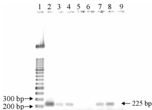
FIGURE 2. Agarose gel depicting amplification of type C toxin gene from DNA extracted from tilapia gastrointestinal contents seeded with multiple dilutions of Clostridium botulinum type C cells (SS36). Lanes: 1, 100-bp DNA ladder (Roche); 2, 96-SAC positive control; 3, 1.0 \times 10^5 cells; 4, 7.5 \times 10^4 cells; 5, 5.0 \times 10^4 cells; 6, 2.5 \times 10^4 cells; 7, 1.5 \times 10^4 cells; 8, 1.0 \times 10^4 cells; 9, no template control.
