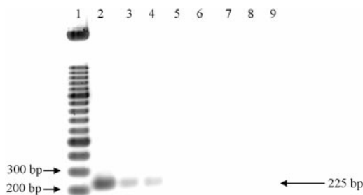
FIGURE 1. Agarose gel depicting amplification of type C toxin gene from DNA extracted from tilapia gastrointestinal contents seeded with multiple dilutions of Clostridium botulinum type C cells (SS36). Lanes: 1, 100-bp DNA ladder (Roche); 2, 96-SAC positive control; 3, 1.0 \times 10^5 cells; 4, 7.5 \times 10^4 cells; 5, 5.0 \times 10^4 cells; 6, 2.5 \times 10^4 cells; 7, 1.5 \times 10^4 cells; 8, 1.0 \times 10^4 cells; 9, no template control.
