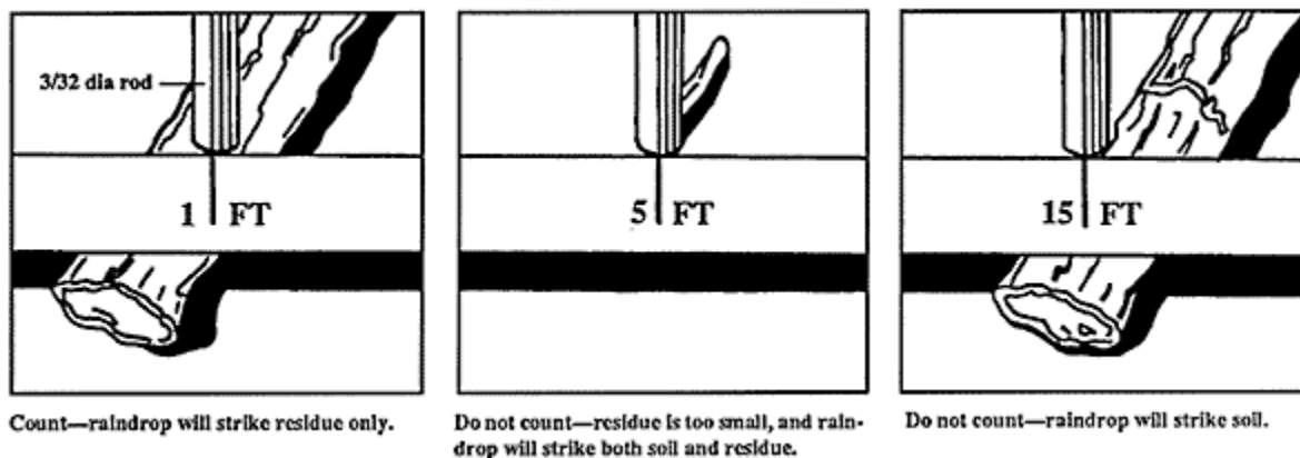
Figure 4. Measuring tape and 3/32 inch diameter rod being used to determine whether or not to count a piece of residue.
