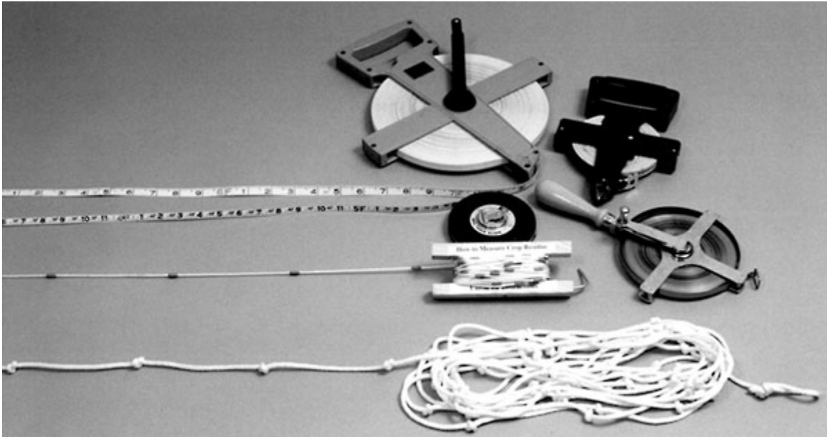
Figure 1. Measuring devices used for determining percent residue cover: tape measures; specially made cord with attached plastic beads; and knotted rope. For convenience, there should be 100 clearly visible marks on the measuring device.
