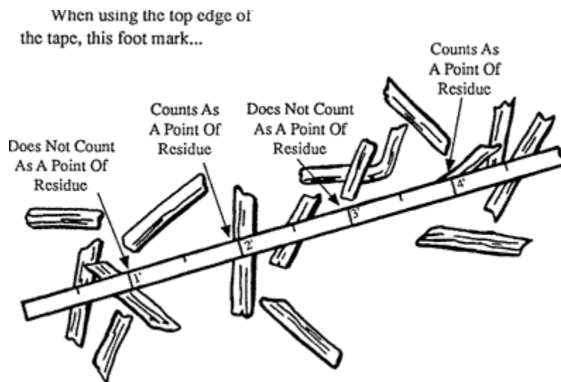
Figure 2 (above). While consistently looking at only one side of the measuring device, count only those marks that have a piece of residue beneath them.
