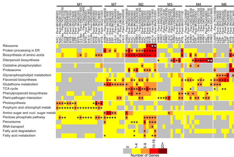
FIGURE 3 | Target TF subnetwork analysis. Modules and target TFs with family and gene id. are shown at the top of the figure. KEGG pathways showing subnetwork enrichment are shown on the left. The number of genes associated with individual TFs in each KEGG pathway are color coded, from gray – no genes to brown – >20 genes. Asterisks denote significant enrichment within the subnetwork at P \leq 0.05 .
