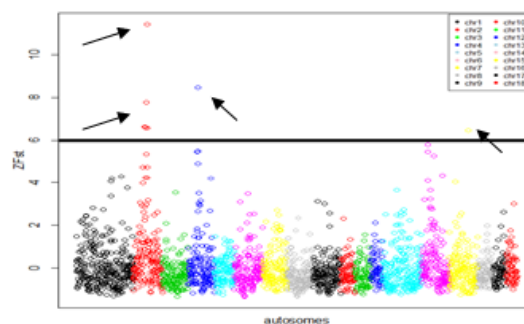
Figure 1: Plot of the normalized Fst (ZFst) values, represented by dots. Each autosome has a different color, as indicated in the legend. The black horizontal line represents the threshold above which a dot is significantly divergent
