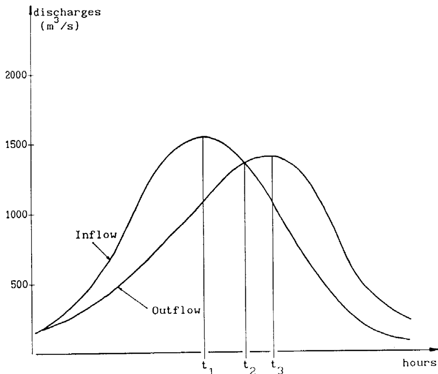
Fig. 1. Typical flood hydrographs for a river reach, with t_1 < t_2 < t_3 .
