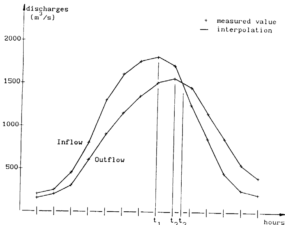
Fig. 2. Frequently observed scenario of flood hydrographs at discrete time steps and their interpolations, with t_1 < t_3 < t_2 .
