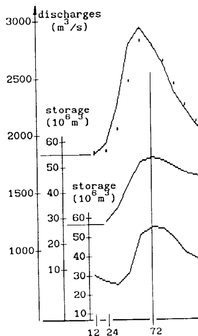
Fig. 3. Synchronous discharges of the River Dunaujvaros (lower station, dots) in discrete time steps and the estimated storage ( S_e ).
