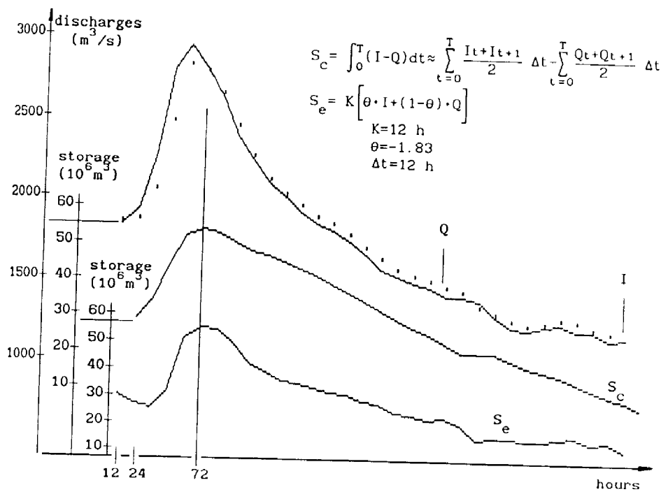
Fig. 3. Synchronous discharges of the River Danube at Budapest (upper station, continuous line) and at Dunaujvaros (lower station, dots) in discrete time steps ( \Delta t = 12 h) as well as the calculated ( S_c ) and estimated storage ( S_e ).
