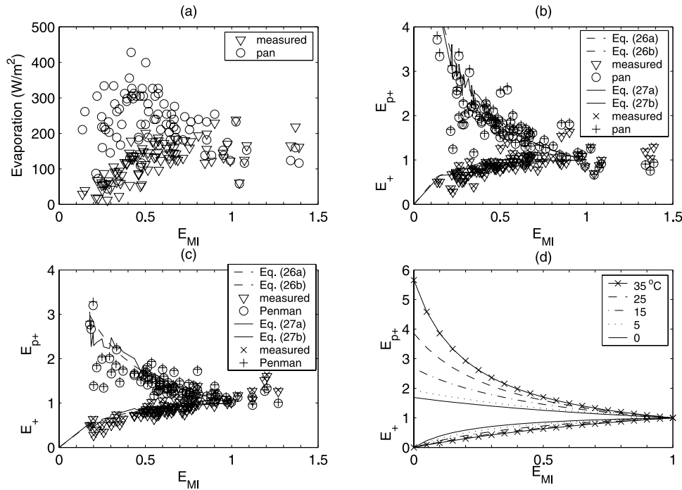
Figure 1. (a) Daily actual ( LE ) and pan evaporation ( LE_{pan} ) data for 1987 and 1989 near Manhattan, KS. E_{MI} = LE/LE_{pan} . (b) LE_w -normalized values of actual ( E_+ ) and pan evaporation ( E_{p+} ) with c = 1.18 (hollow symbols) and c = 1.15 . The curves represent (26) and (27) with b = 9.45 and \varepsilon = 4.71 , respectively, E_{MI} = LE/LE_{pan} . (c) LE_w -normalized values of actual ( E_+ ) and Penman-equation (PM) evaporation ( E_{p+} ) with c = 1.2 (hollow symbols) and c = 1.17 . The curves represent (26) and (27) with b = 4.21 and \varepsilon = 2.24 , respectively, E_{MI} = LE/LE_{PM} . (d) Dimensionless graph of the complementary relationship as predicted by (27) with \varepsilon = 1 .
