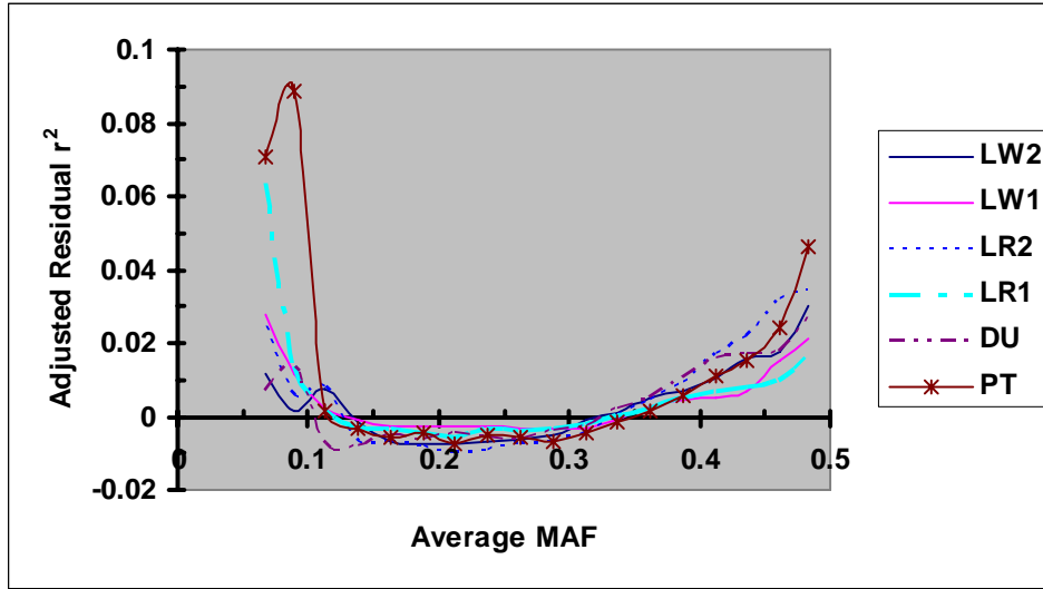
Figure 7. Average r^2 adjusted by recombination rate and r^2_{H0} as a function of average frequency of the minor alleles at each pair of SNPs in six pig lines. The breed origins of all lines were described in Table 1.
