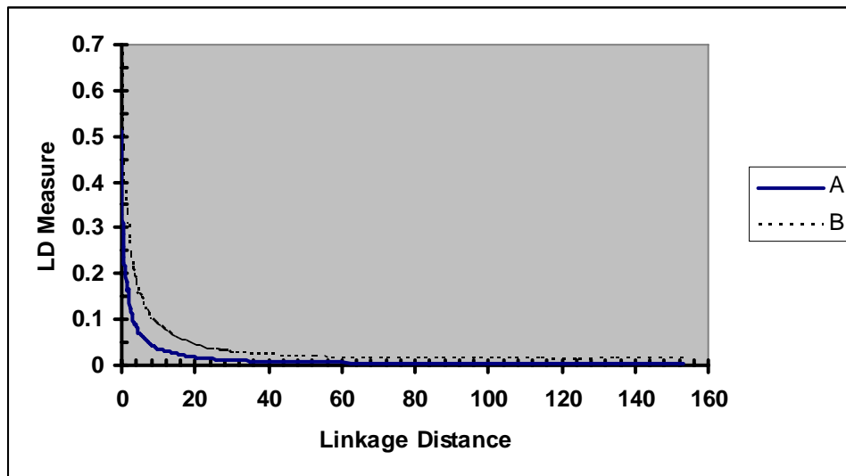
Figure 8. Average of the observed LD measures adjusted by recombination rate as a function of map distance between two SNPs of each pair. A, r^2 ; B, r^2/r^2_{max} as defined in Eq. 5.
