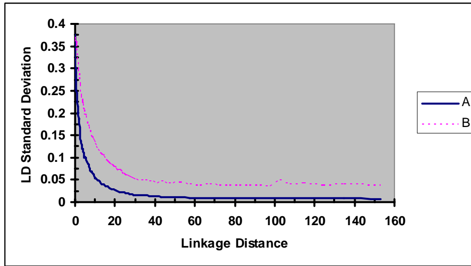
Figure 9. Standard deviation of the observed LD measures adjusted by recombination rate as a function of map distance between two SNPs of each pair. A, r^2 ; B, r^2/r^2_{\max} as defined in Eq. 5.
