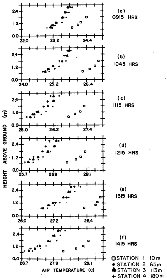
FIG. 5. Temperature profiles at varying distances from the leading edge of an irrigated alfalfa field at Mead, NE, 21 June 1976.
