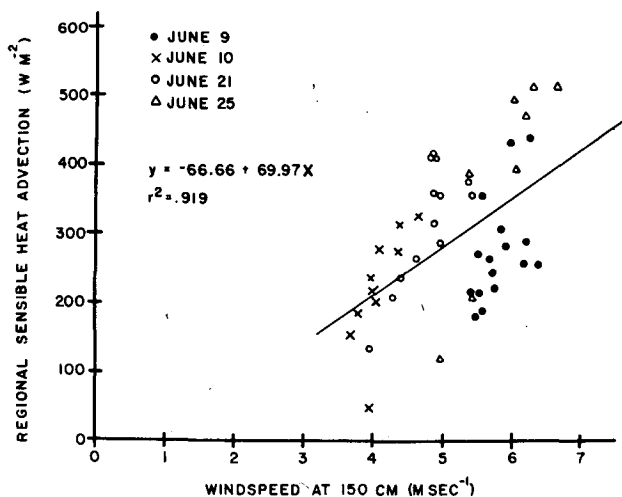
FIG. 10. Dependence of regional sensible heat advection on wind speed above irrigated alfalfa at Mead, NE.
