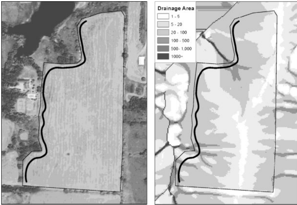
Figure 6. Example 6.7 ha study site with a hypothetical 3 m wide vegetative filter strip (drainage/VFS area ratio = 41) (corrected for actual drainage area to the strip). Flow accumulation along entire filter strip used in flow distribution predictions
