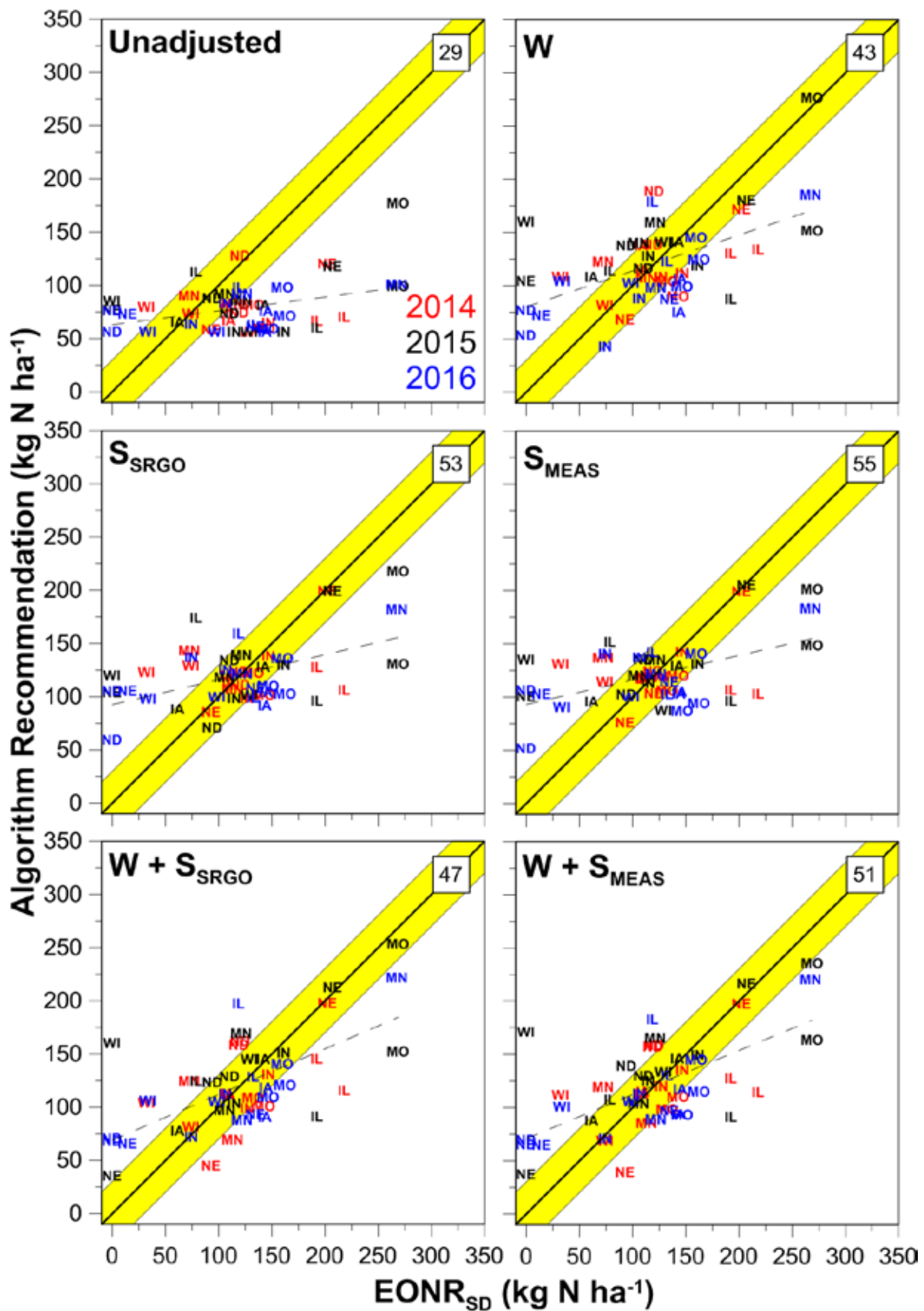
Fig. 2. For corn receiving 45 \text{ kg N ha}^{-1} at planting, performance of the University of Missouri active-optical reflectance sensor algorithm ( \text{ALG}_{\text{MU}} ) for making N fertilizer recommendations, with and without weather (W) and soil (USDA SSURGO [ \text{S}_{\text{SRGO}} ]; Measured [ \text{S}_{\text{MEAS}} ]) adjustments, by comparing the recommendation to economic optimal N rate ( \text{EONR}_{\text{SD}} ). Points near the 1:1 line dissecting the graph indicate sites where the AORS algorithm was relatively accurate in recommending an N rate approximate to \text{EONR}_{\text{SD}} . Sites that fell within the yellow shaded region are those within 34 \text{ kg N ha}^{-1} of \text{EONR}_{\text{SD}} , with the percentage of the 49 sites within this region indicated in the top right corner of each graph.
