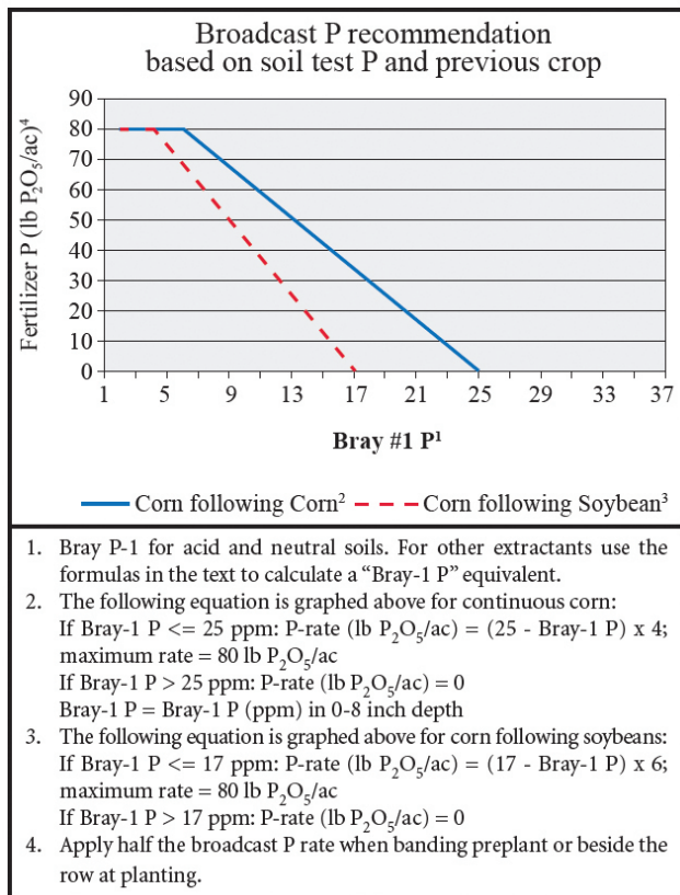
Figure 2. Broadcast P recommendation based on soil test P and the previous crop.
