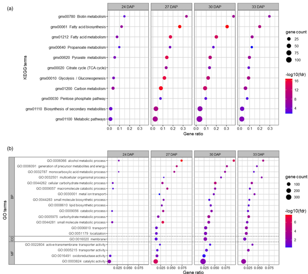
Figure 5 KEGG pathway enrichment and GO functional classification of differentially expressed genes in WD events grown in a greenhouse. Statistically significantly enriched ( \text{FDR} < 0.05 ) KEGG pathways in (a) and Gene Ontology terms in (b) are shown for the DEGs identified at each developmental stage. Three GO categories are presented, including Biological Processes (BP), Cellular Compartment (CC), and Molecular Function (MF). The gene count represents the number of non-unique DEGs enriched in a pathway. The absence of a dot indicates the pathway was not significantly enriched in that developmental stage. Gene ratio was calculated as the number of DEGs involved in a pathway divided by the total number of soybean genes in the pathway. Enriched GO terms resulting from AgriGOv2 were consolidated into fewer non-redundant GO terms using Revigo ( http://revigo.irb.hr ) for visualization purposes in (b) ( \text{FDR} < 0.05 ). DAP: days after pollination. TCA: tricarboxylic acid cycle.
