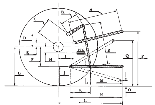
HITCH DIMENSIONS AS TESTED—NO LOAD
