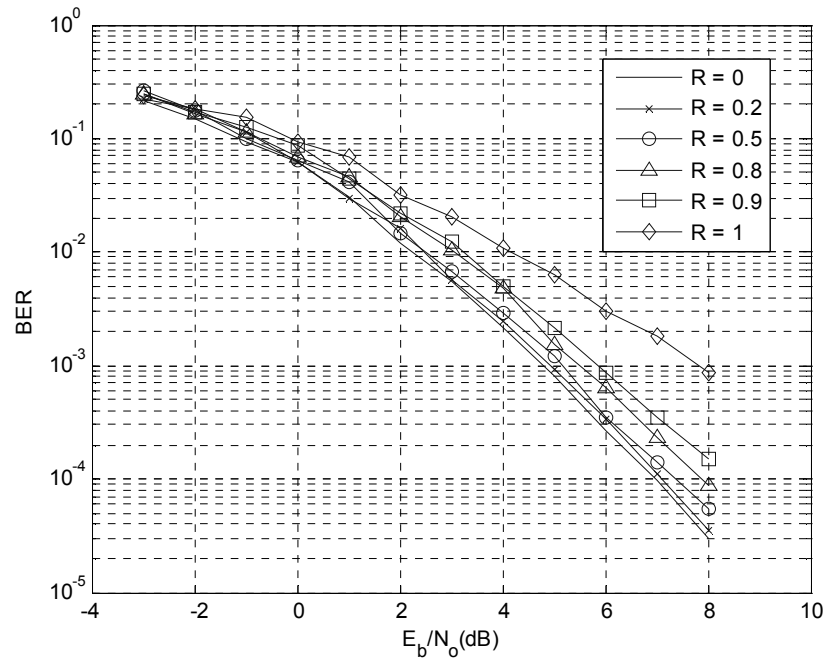
Fig. 4.6 Simulation BER of CCC with K_{10}=K_{20}=K_{30}=0.5 , K_{12}=K_{13}=0.5 , in correlated channel.
