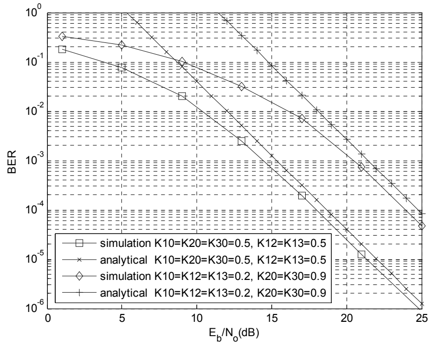
Fig. 4.4 Analytical and simulation BER of MRC.
