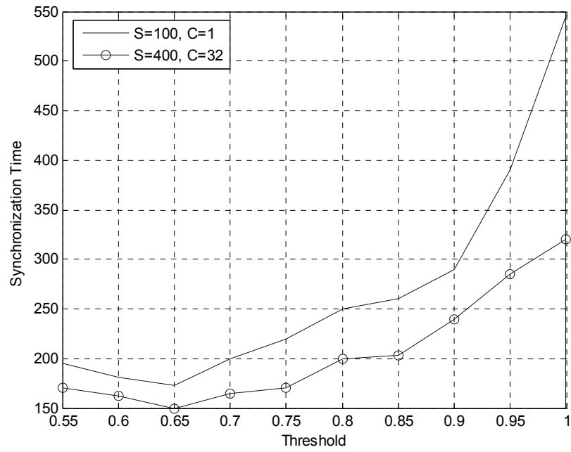
Fig. 3.14 Synchronization time 2L_1+L_2 (bits) improvement with parallel correlators and a larger sequence pool for N = 64 .
