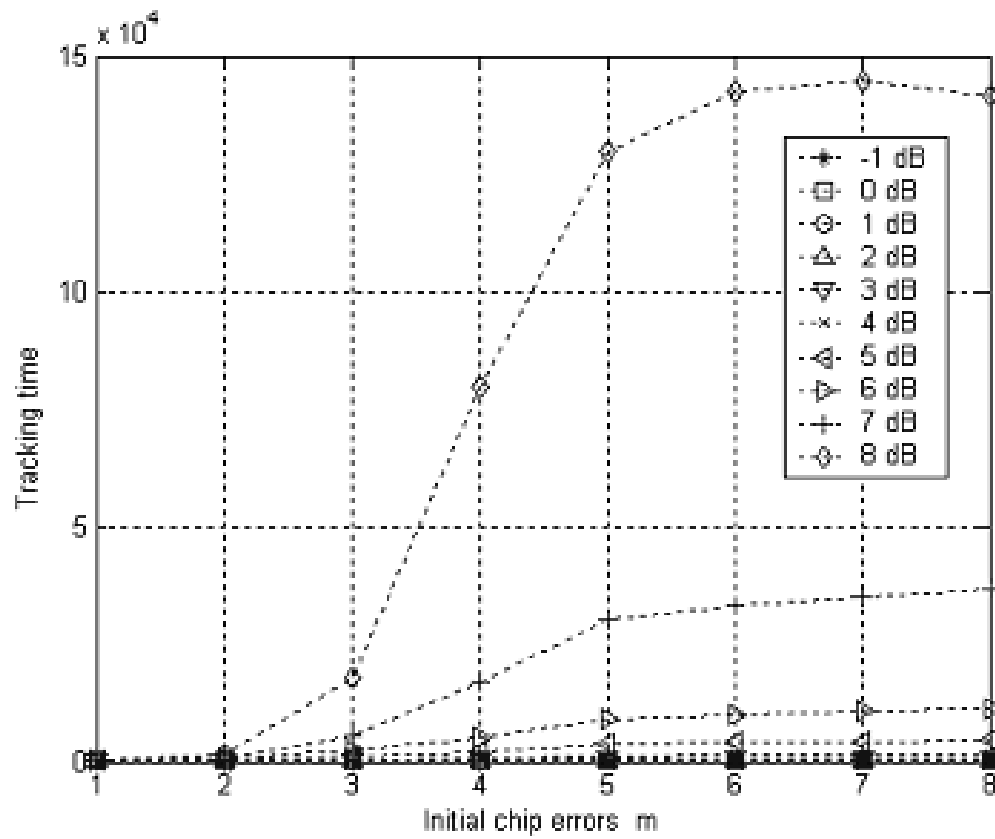
Fig. 3.6 Simulation of tracking time L_2 (bits) for N = 8 .
