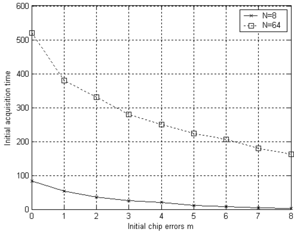
Fig. 3.3 Initial acquisition time 2L_1 (bits) for N = 8, 64 .
