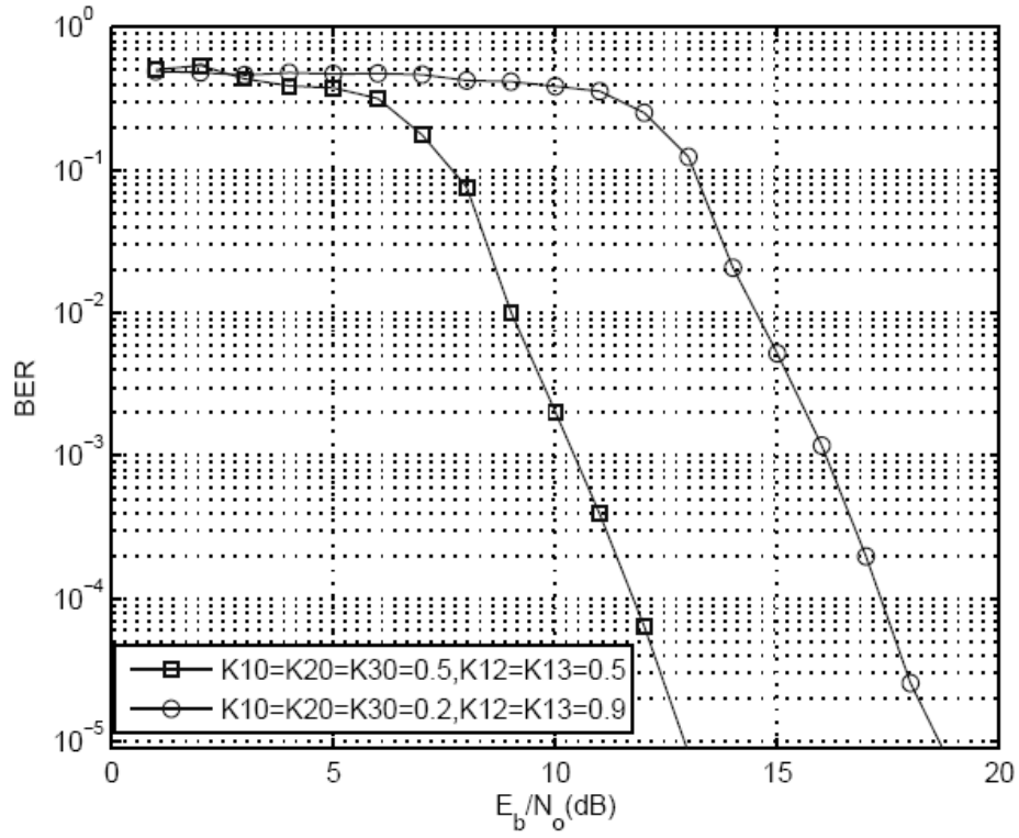
Fig. 5.4. Simulation BER of SESS-CD, 64 chips/bit.
