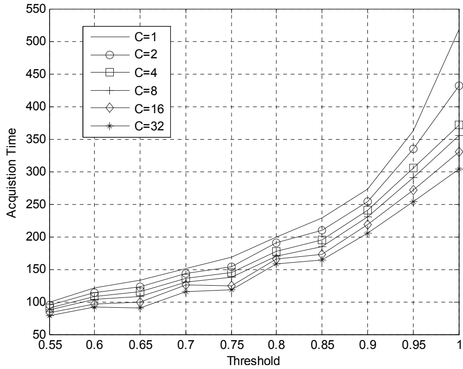
Fig. 3.11 Initial acquisition time 2L_1 (bits) with parallel correlators for N = 64 .
