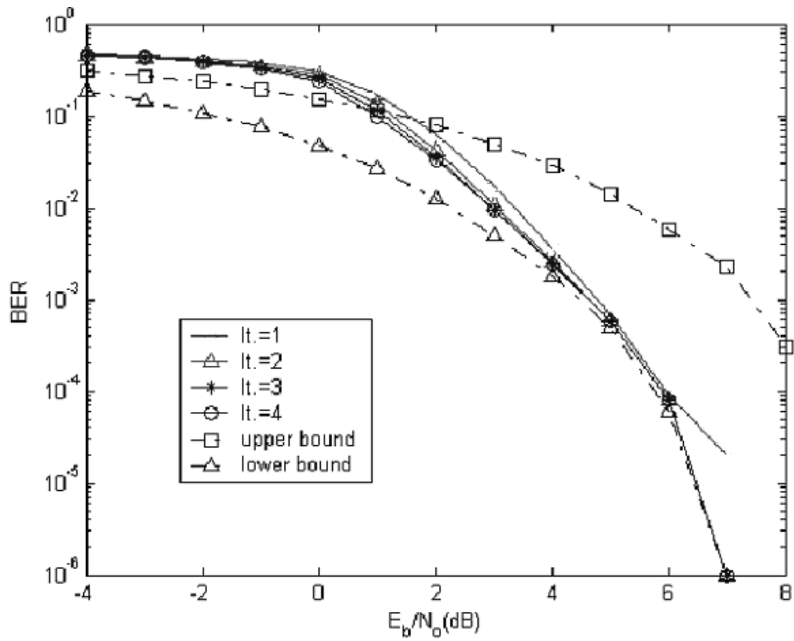
Figure 2.4 BER performance of iteration detector from Iteration 1-4 iterations
