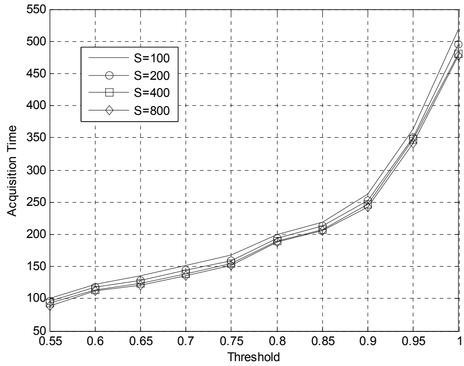
Fig. 3.12 Initial acquisition time 2L_I (bits) with larger sequence pool for N = 64 .
