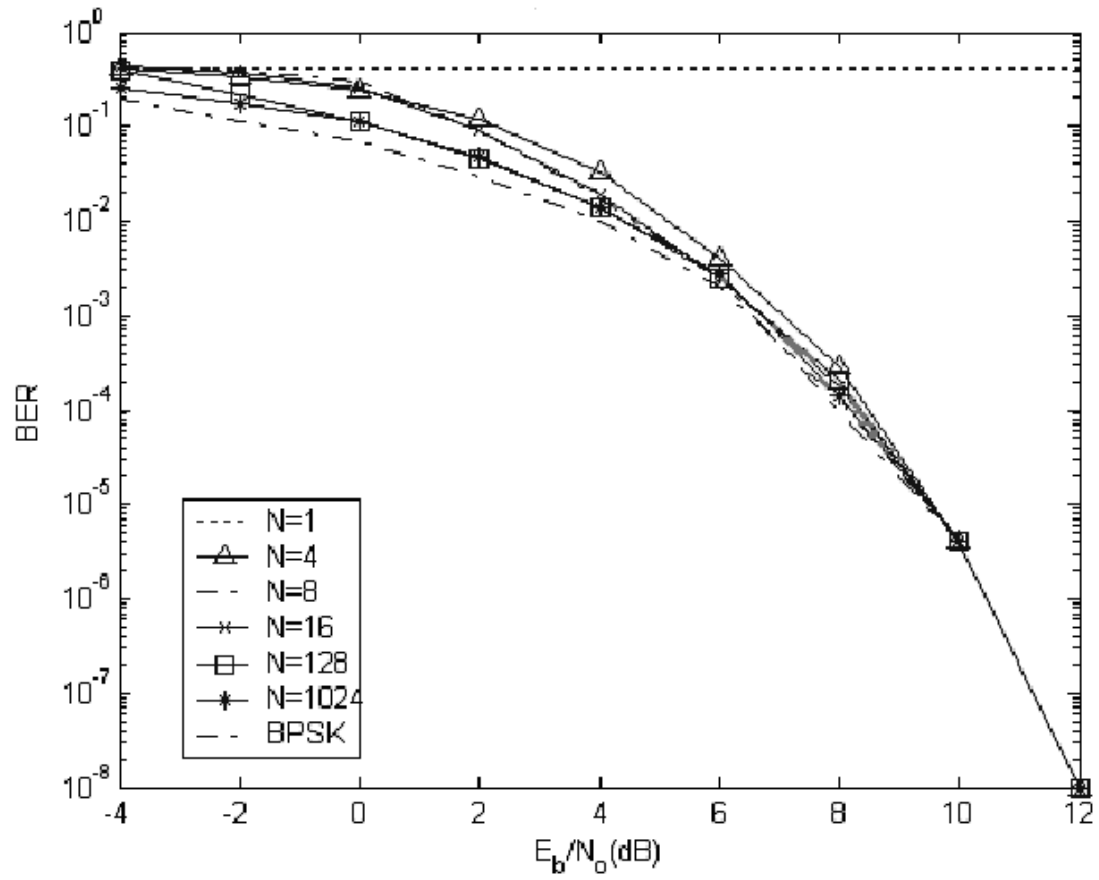
Figure 2.2 Self-encoding feedback detection performance.
