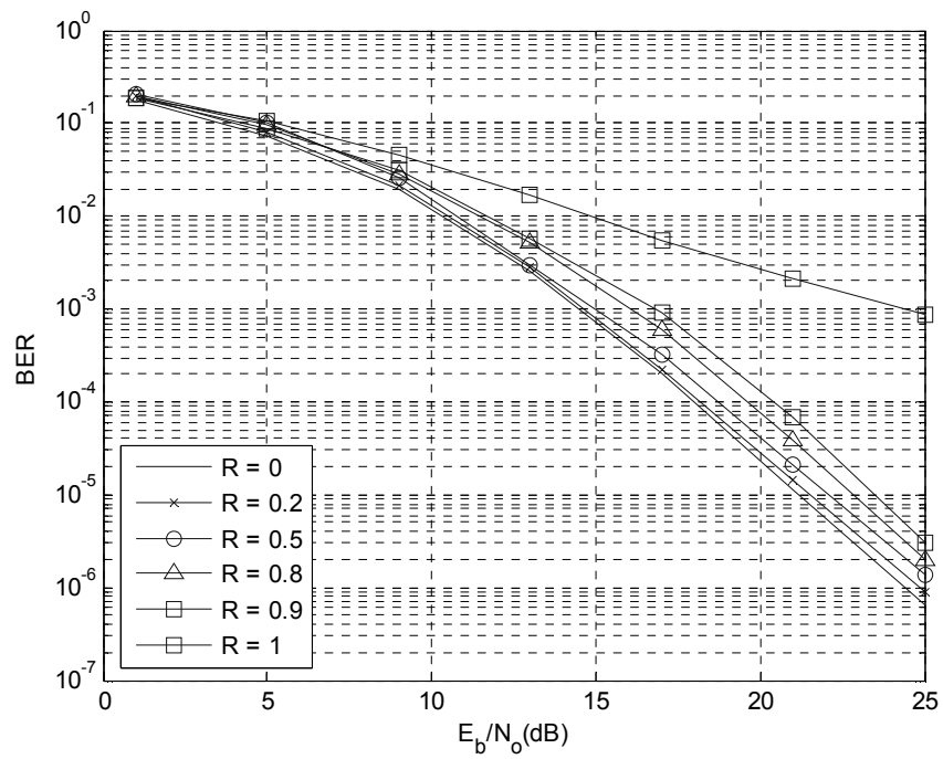
Fig. 4.5 Simulation BER of MRC with K_{10} = K_{20} = K_{30} = 0.5 , K_{12} = K_{13} = 0.5 , for various correlation values of correlated channel.
