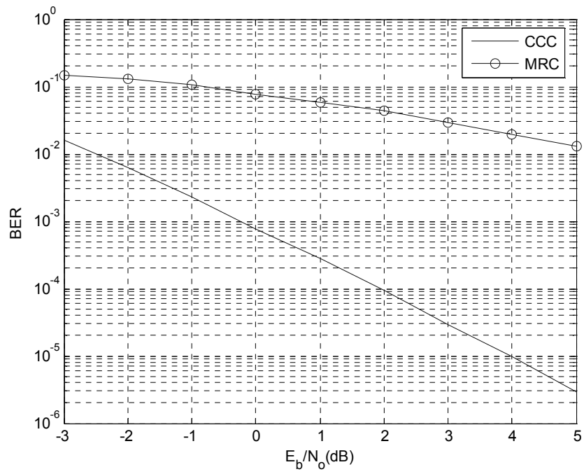
Fig. 4.3 Simulation BER, CCC and MRC, K_{10}=K_{20}=K_{30}=1 , K_{12}=K_{13}=1 .
