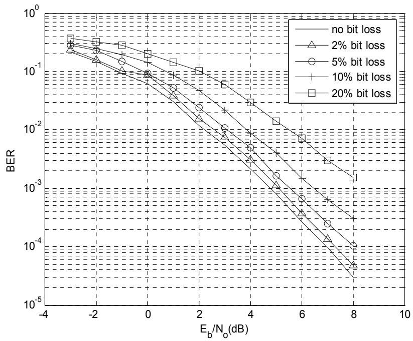
Fig. 4.8 Simulation BER of CCC with K_{10}=K_{20}=K_{30}=0.5 , K_{12}=K_{13}=0.5 , for various bit loss percentages.
