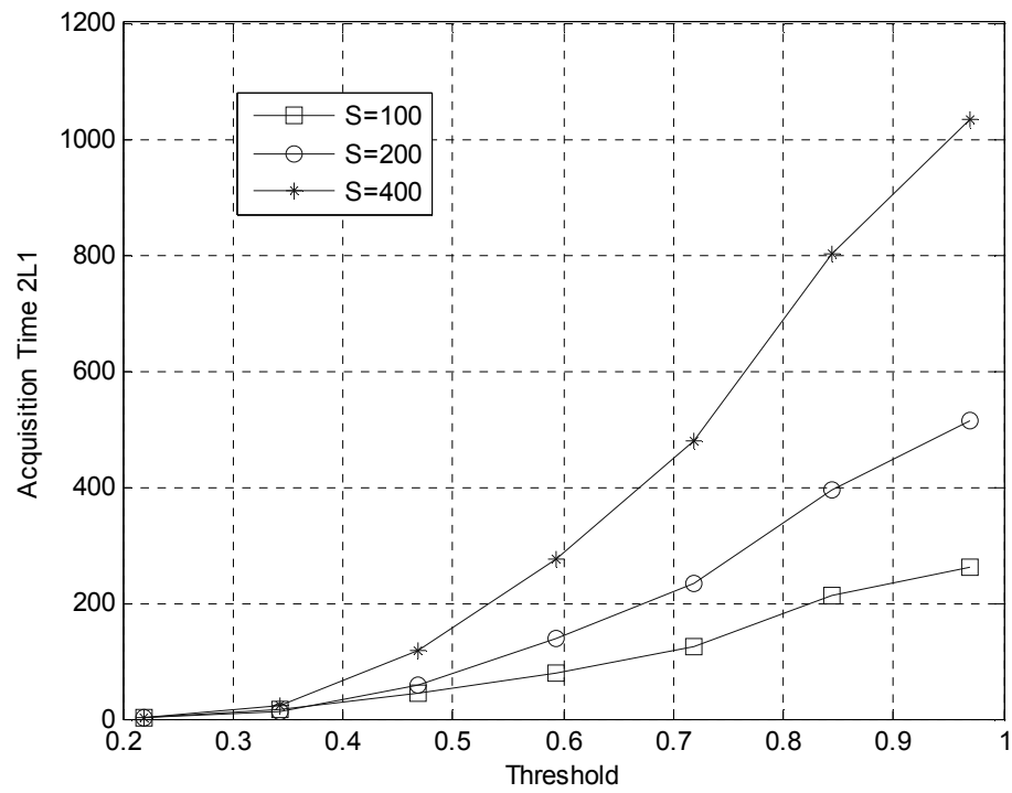
Fig. 3.13 Initial acquisition time 2L_1 (bits) with larger sequence pools for cross-over=90% and mutation=5%
