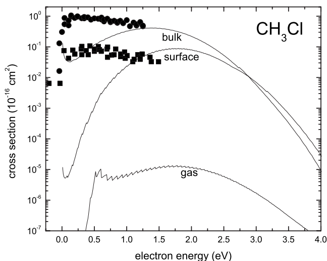
FIG. 6. DEA cross sections for the CH 3 Cl molecule. Experimental data: squares, surface; circles, bulk.
