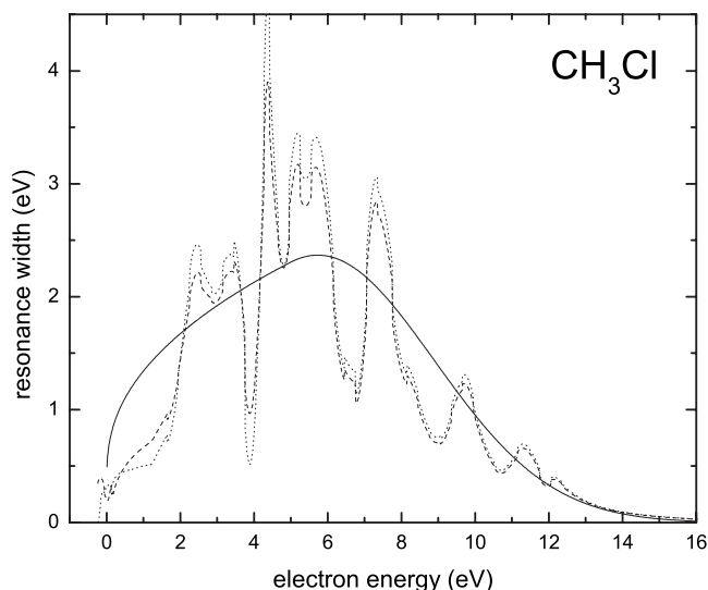
FIG. 4. Resonance width for the CH 3 Cl molecule at the equilibrium internuclear separation: solid line, gas-phase width; dashed line, molecules at the surface of the Kr film; dotted line, molecules buried under the surface at the distance 50 a.u.
