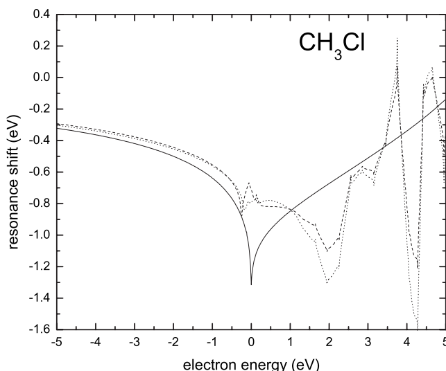
FIG. 5. Resonance shift for the CH 3 Cl molecule at the equilibrium internuclear separation. The curve notation is the same as in Fig. 4.
