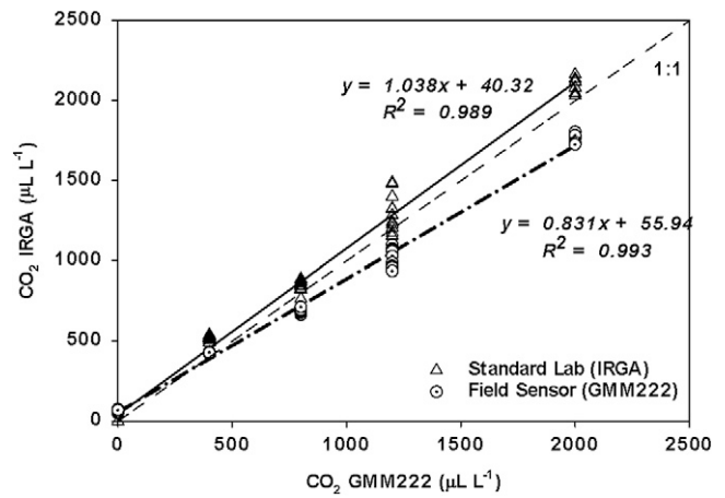
Fig. 3. Measurements from an infrared gas analyzer (IRGA; Model ADC-225 MK3, Analytical Development Company, Hoddeson, UK) and a single CO 2 sensor (Model GMM222, Vaisala, Finland) in five known atmospheric concentrations of CO 2 (0, 400, 800, 1200, and 2000 μL L -1 ). The dashed line is a 1:1 concentration.
