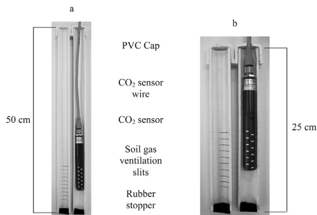
Fig. 1. Cut-away view of CO 2 sensors inside PVC tubing. The tubing was inserted vertically into the soil, putting the CO 2 sensors at (a) 38 cm and (b) 15 cm deep.
