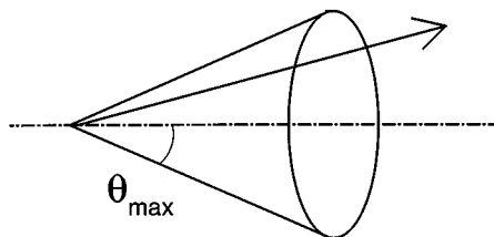
FIG. 1. Definition of the steric hindrance angle \theta_{\max} . The direction of the vector (shown as an arrow in the figure) describing the relative orientation of the two fragments in the transition state configuration is confined to the solid angle region that is defined by (using spherical coordinates) 0 \leq \phi < 2\pi and 0 \leq \theta \leq \theta_{\max} , and is shown as a cone (after Ref. 3).
