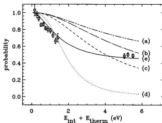
FIG. 2. Relative cross section (or reaction probability) of reaction (10) as a function of internal energy (including an amount of about 91 meV of thermal energy representing initial rotational and kinetic energy). The vertical axis gives the reaction probability, defined as P_j = \sigma_j / \sigma_{\text{LGS}} (see text). The squares are the experimental results of Ref. 5, scaled to fit the calculations. The five curves show the results of RRKM calculations with restrictions. (a) (dash-dot-dot curve) Result obtained when all degrees of freedom are active. (b) (dash-dot curve) One vibration of 3420 \text{ cm}^{-1} in the products' transition state is inactive. (c) (dashed curve) One vibration of 1330 \text{ cm}^{-1} in the products' transition state is inactive. (d) (dotted curve) Three vibrations of 1330 \text{ cm}^{-1} in the products' transition state are inactive. (e) (solid curve) This is the result obtained for two inactive vibrations of 1615 \text{ cm}^{-1} in the reactants' transition state and one inactive vibration of 3420 \text{ cm}^{-1} together with increased rotational constants in the products' transition state: B_{\text{eff}}/B = 2.35 , which implies \theta_{\max} = 81^\circ .
