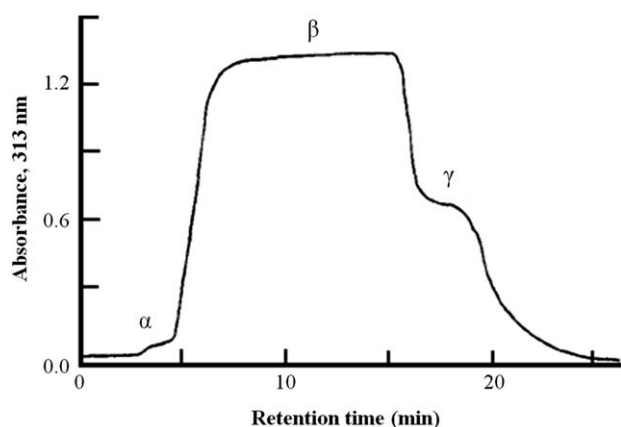
Fig. 3 Chromatogram obtained by high-performance frontal analysis (HPFA) for a mixture of warfarin and HSA. The sample was a mixture of 100 \mu\text{M} warfarin plus 2 \text{g L}^{-1} HSA that was injected onto a 30 cm \times 3.9 mm I.D. size-exclusion column. Reproduced with permission from ref. 60.
