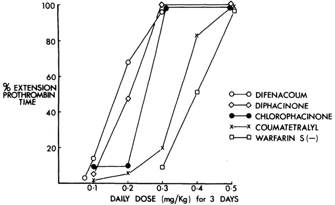
Figure 2. The effect on the extension of male Wistar rats prothrombin times following three daily oral administrations of various rodenticides.
