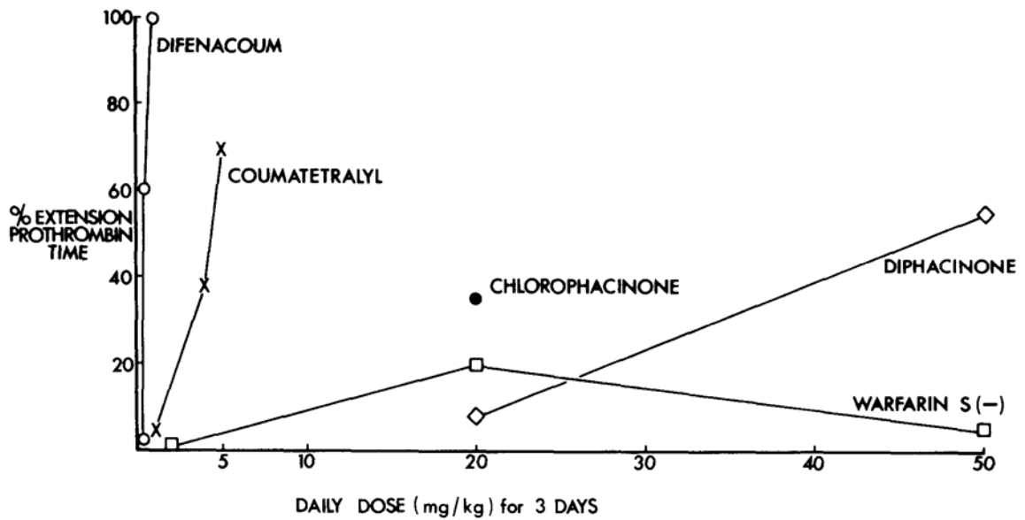
Figure 3. The effect on the extension of prothrombin times of homozygous resistant (Welsh strain) male rats following three daily oral administrations of various rodenticides.
