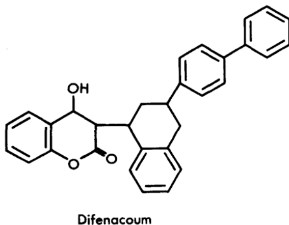
Figure 1. Comparative structures of three rodenticides.
